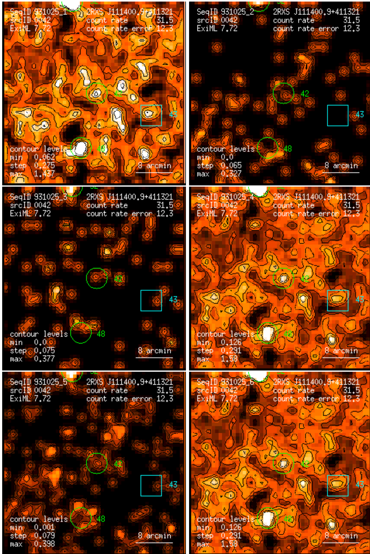
Figure 42: RASS 931025: detection 0042: band rate images, Gaussian filter: (1) PSPC channels 11 – 41, (2) 52 – 90, (3) 91 – 201, (4) 11 – 235, (5) 52 – 201, (6) 11 – 201. Broad band rates in counts/ks. Band rate contour levels in counts/ks/arcmin 2 .
