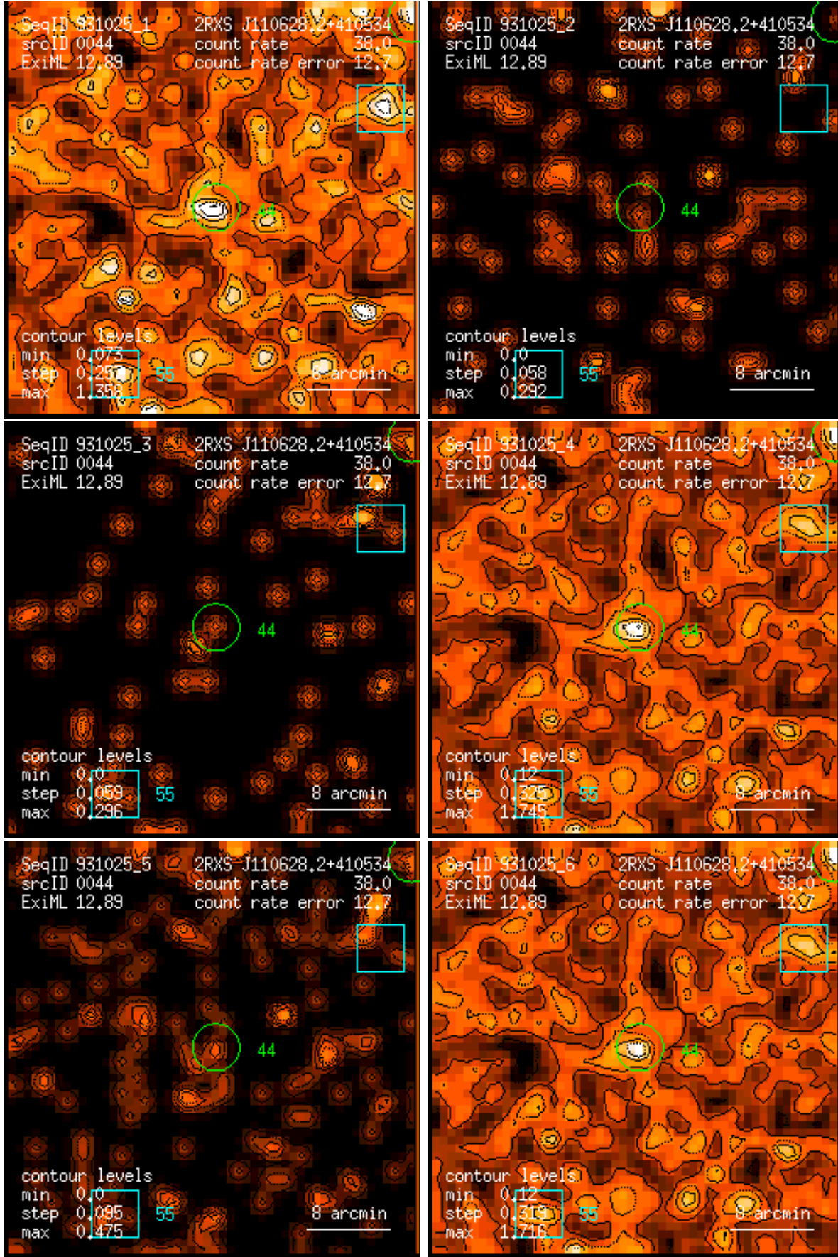
Figure 44: RASS 931025: detection 0044: band rate images, Gaussian filter: (1) PSPC channels 11 – 41, (2) 52 – 90, (3) 91 – 201, (4) 11 – 235, (5) 52 – 201, (6) 11 – 201. Broad band rates in counts/ks. Band rate contour levels in counts/ks/arcmin 2 .
