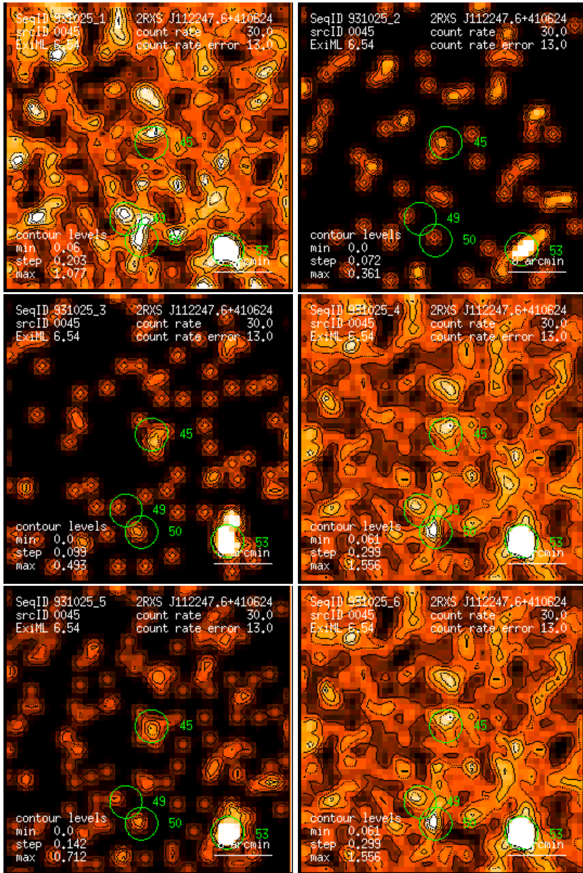
Figure 45: RASS 931025: detection 0045: band rate images, Gaussian filter: (1) PSPC channels 11 – 41, (2) 52 – 90, (3) 91 – 201, (4) 11 – 235, (5) 52 – 201, (6) 11 – 201. Broad band rates in counts/ks. Band rate contour levels in counts/ks/arcmin 2 .
