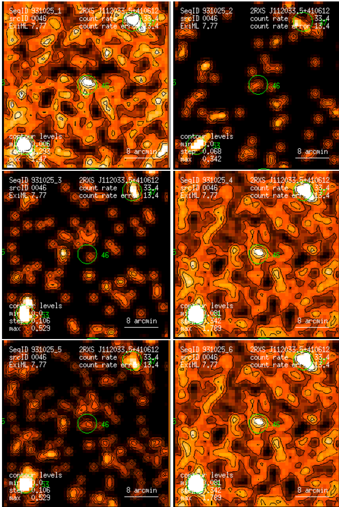
Figure 46: RASS 931025: detection 0046: band rate images, Gaussian filter: (1) PSPC channels 11 – 41, (2) 52 – 90, (3) 91 – 201, (4) 11 – 235, (5) 52 – 201, (6) 11 – 201. Broad band rates in counts/ks. Band rate contour levels in counts/ks/arcmin 2 .
