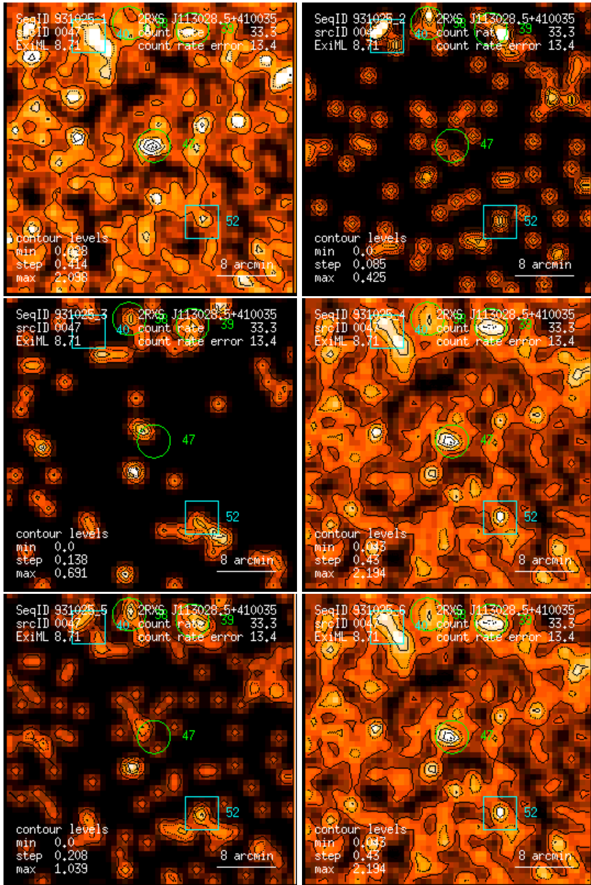
Figure 47: RASS 931025: detection 0047: band rate images, Gaussian filter: (1) PSPC channels 11 – 41, (2) 52 – 90, (3) 91 – 201, (4) 11 – 235, (5) 52 – 201, (6) 11 – 201. Broad band rates in counts/ks. Band rate contour levels in counts/ks/arcmin 2 .
