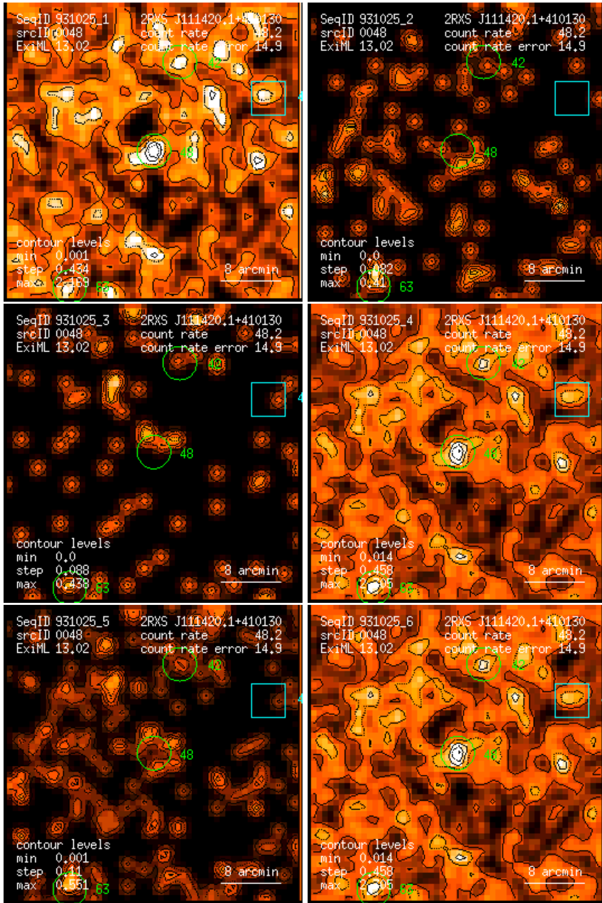
Figure 48: RASS 931025: detection 0048: band rate images, Gaussian filter: (1) PSPC channels 11 – 41, (2) 52 – 90, (3) 91 – 201, (4) 11 – 235, (5) 52 – 201, (6) 11 – 201. Broad band rates in counts/ks. Band rate contour levels in counts/ks/arcmin 2 .
