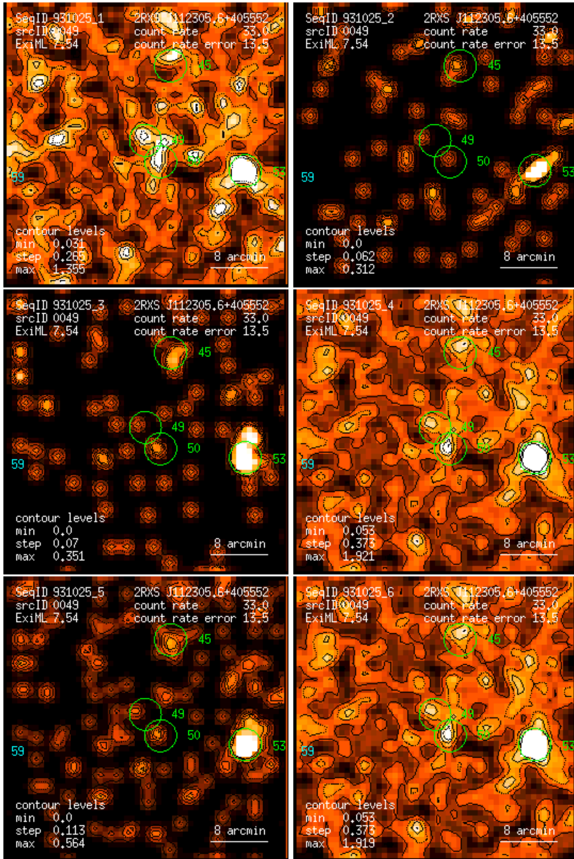
Figure 49: RASS 931025: detection 0049: band rate images, Gaussian filter: (1) PSPC channels 11 – 41, (2) 52 – 90, (3) 91 – 201, (4) 11 – 235, (5) 52 – 201, (6) 11 – 201. Broad band rates in counts/ks. Band rate contour levels in counts/ks/arcmin 2 .
