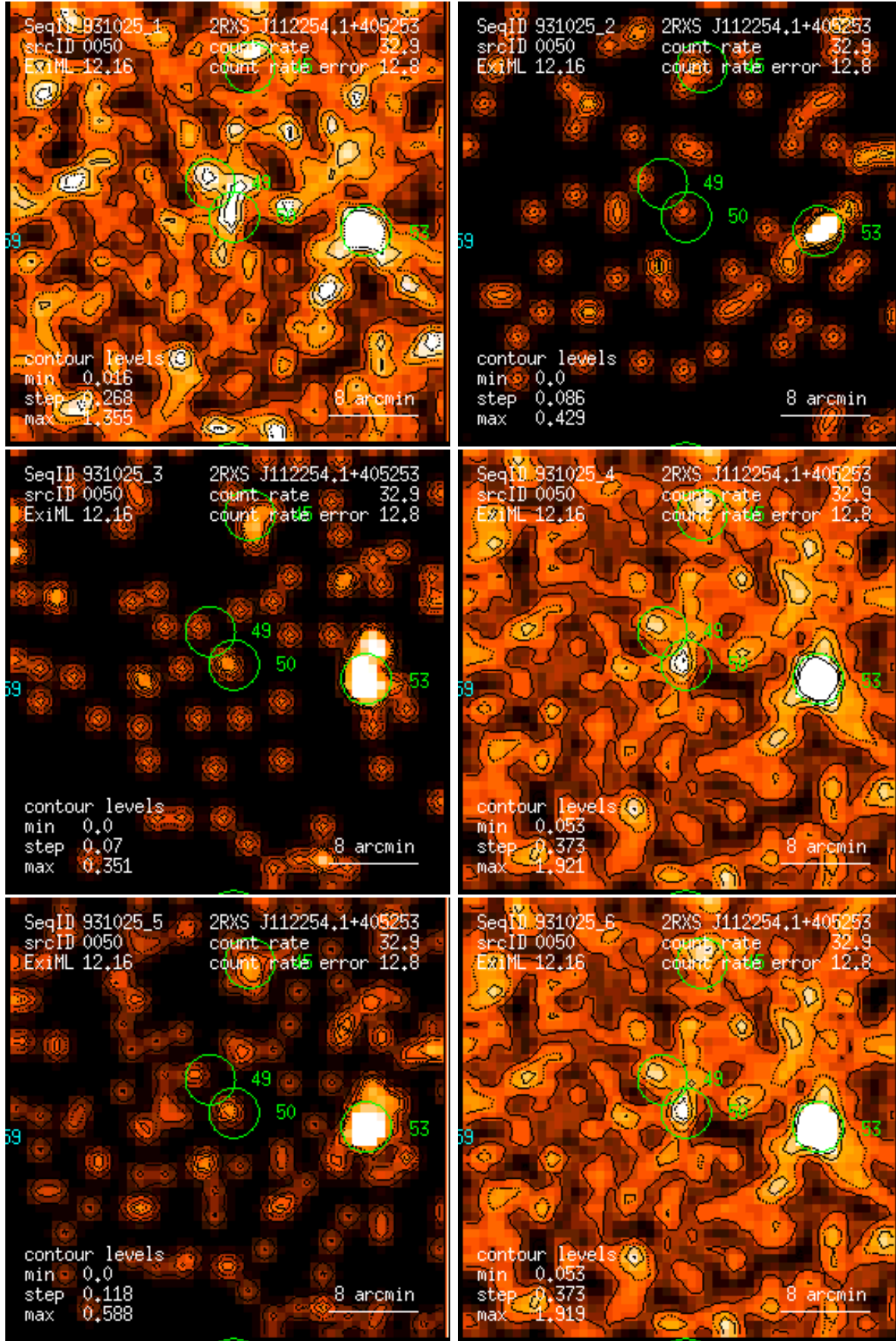
Figure 50: RASS 931025: detection 0050: band rate images, Gaussian filter: (1) PSPC channels 11 – 41, (2) 52 – 90, (3) 91 – 201, (4) 11 – 235, (5) 52 – 201, (6) 11 – 201. Broad band rates in counts/ks. Band rate contour levels in counts/ks/arcmin 2 .
