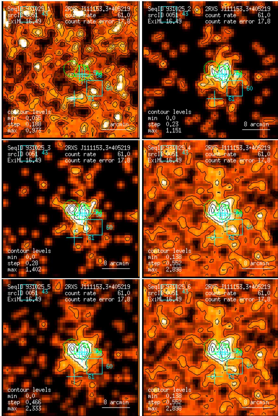
Figure 51: RASS 931025: detection 0051: band rate images, Gaussian filter: (1) PSPC channels 11 – 41, (2) 52 – 90, (3) 91 – 201, (4) 11 – 235, (5) 52 – 201, (6) 11 – 201. Broad band rates in counts/ks. Band rate contour levels in counts/ks/arcmin 2 .
