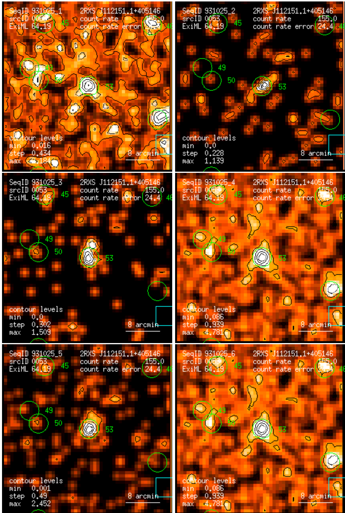
Figure 53: RASS 931025: detection 0053: band rate images, Gaussian filter: (1) PSPC channels 11 – 41, (2) 52 – 90, (3) 91 – 201, (4) 11 – 235, (5) 52 – 201, (6) 11 – 201. Broad band rates in counts/ks. Band rate contour levels in counts/ks/arcmin 2 .
