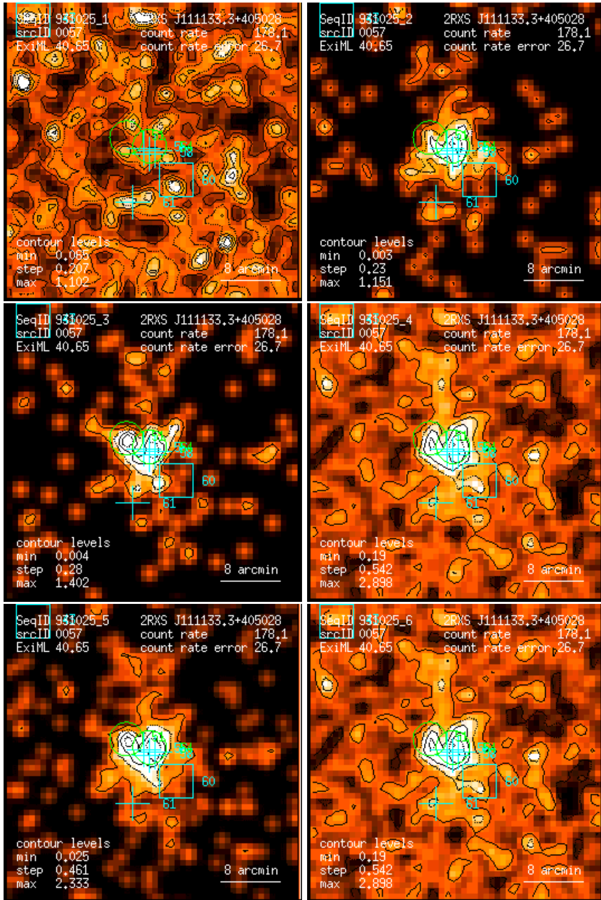
Figure 57: RASS 931025: detection 0057: band rate images, Gaussian filter: (1) PSPC channels 11 – 41, (2) 52 – 90, (3) 91 – 201, (4) 11 – 235, (5) 52 – 201, (6) 11 – 201. Broad band rates in counts/ks. Band rate contour levels in counts/ks/arcmin 2 .
