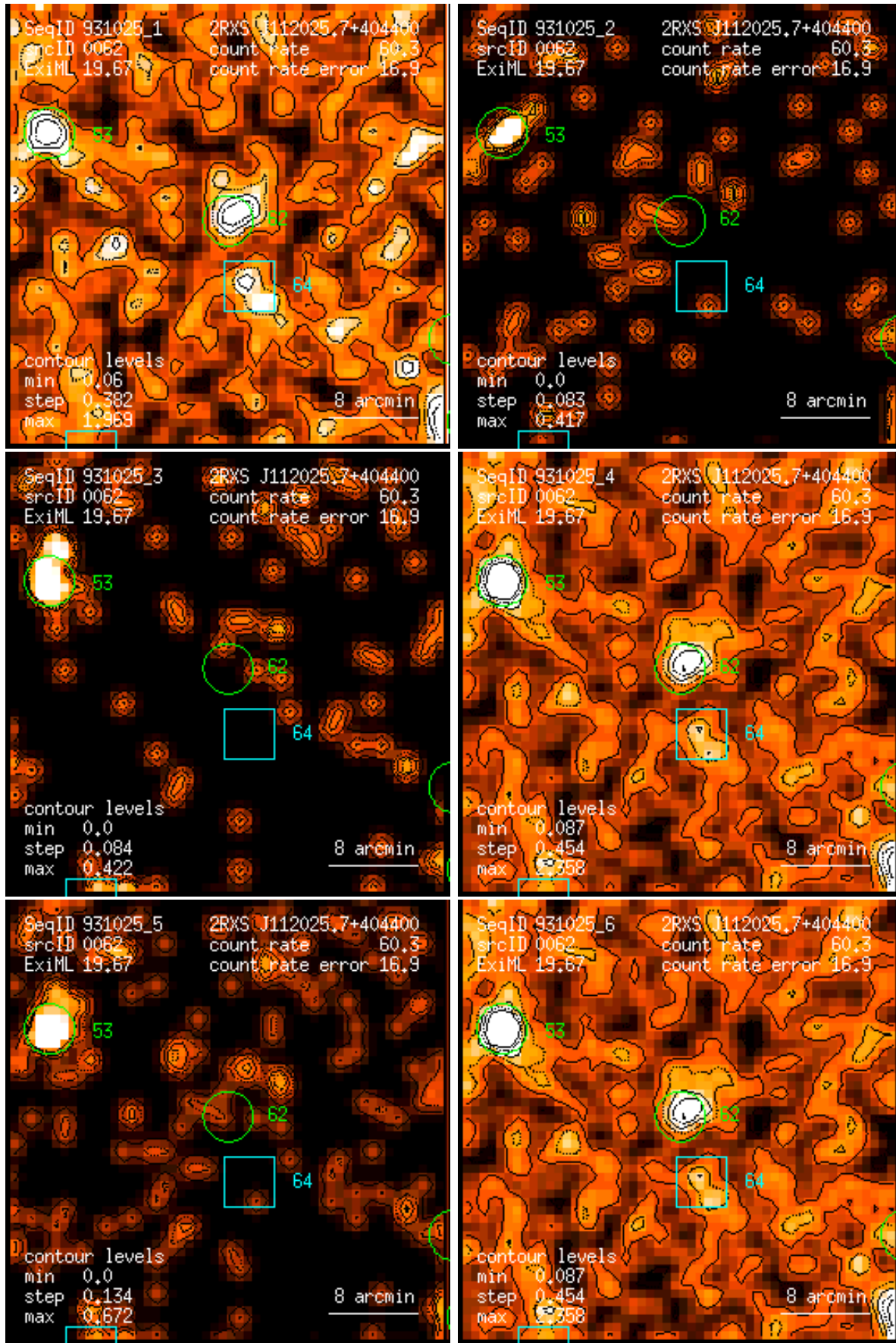
Figure 62: RASS 931025: detection 0062: band rate images, Gaussian filter: (1) PSPC channels 11 – 41, (2) 52 – 90, (3) 91 – 201, (4) 11 – 235, (5) 52 – 201, (6) 11 – 201. Broad band rates in counts/ks. Band rate contour levels in counts/ks/arcmin 2 .
