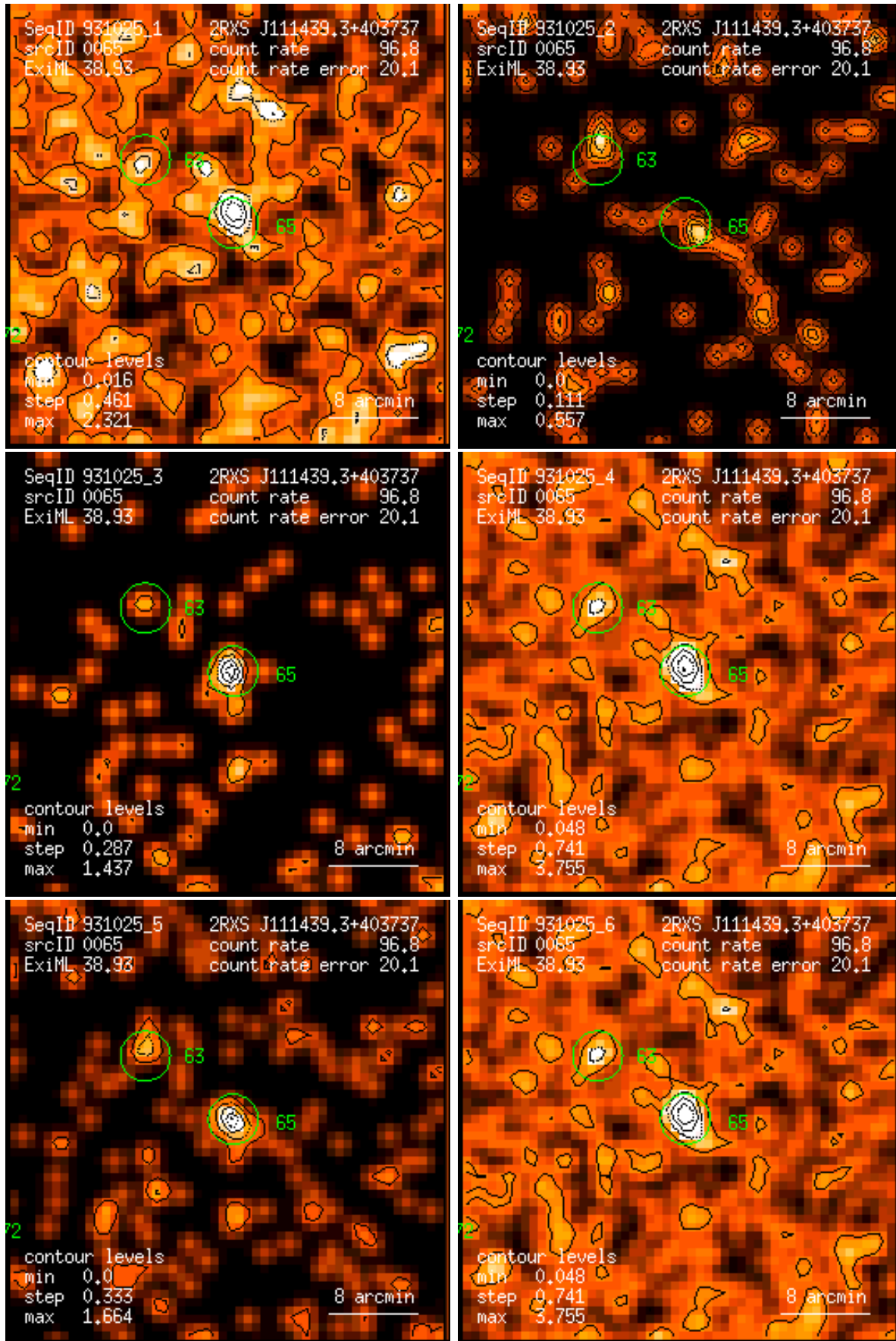
Figure 65: RASS 931025: detection 0065: band rate images, Gaussian filter: (1) PSPC channels 11 – 41, (2) 52 – 90, (3) 91 – 201, (4) 11 – 235, (5) 52 – 201, (6) 11 – 201. Broad band rates in counts/ks. Band rate contour levels in counts/ks/arcmin 2 .
