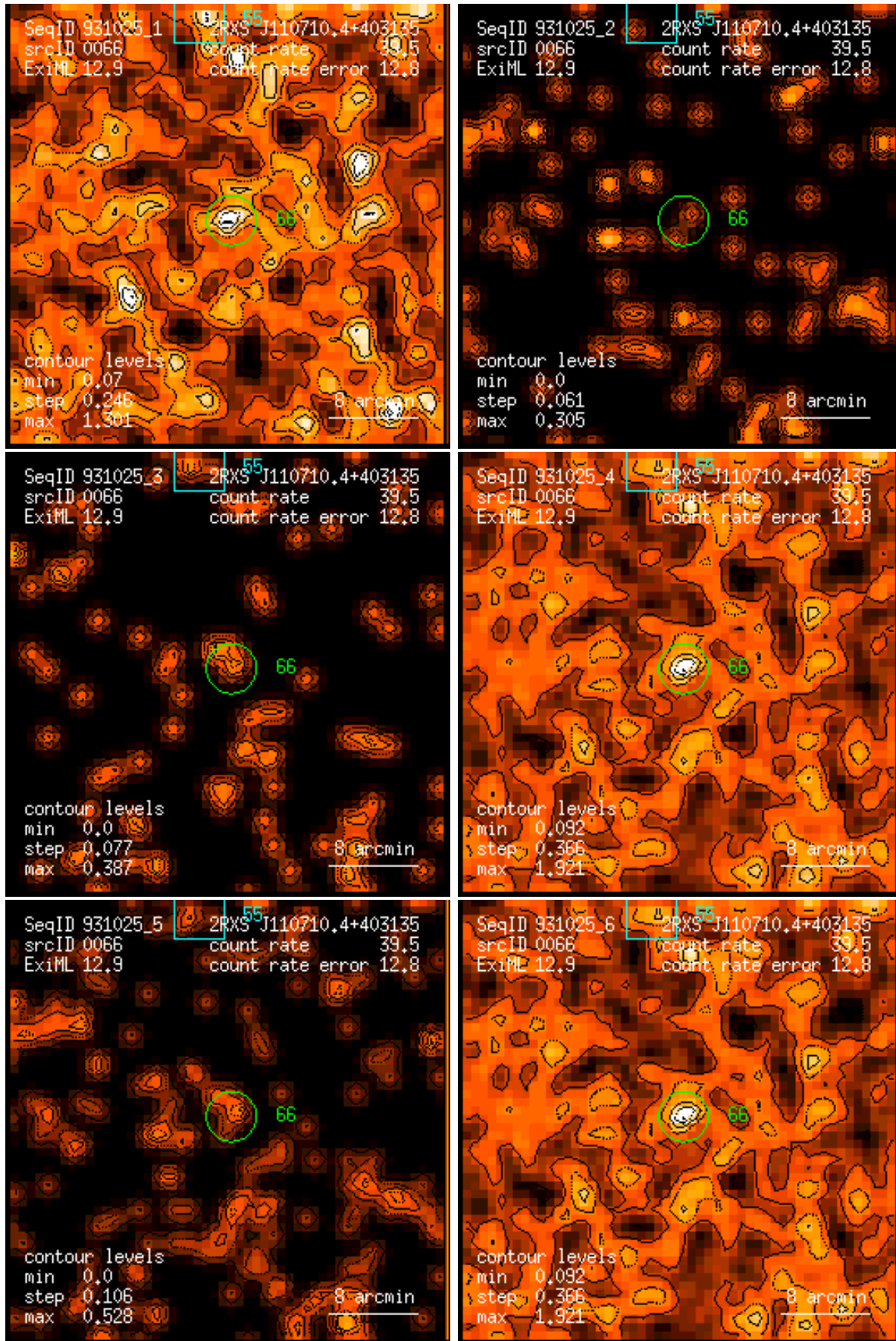
Figure 66: RASS 931025: detection 0066: band rate images, Gaussian filter: (1) PSPC channels 11 – 41, (2) 52 – 90, (3) 91 – 201, (4) 11 – 235, (5) 52 – 201, (6) 11 – 201. Broad band rates in counts/ks. Band rate contour levels in counts/ks/arcmin 2 .
