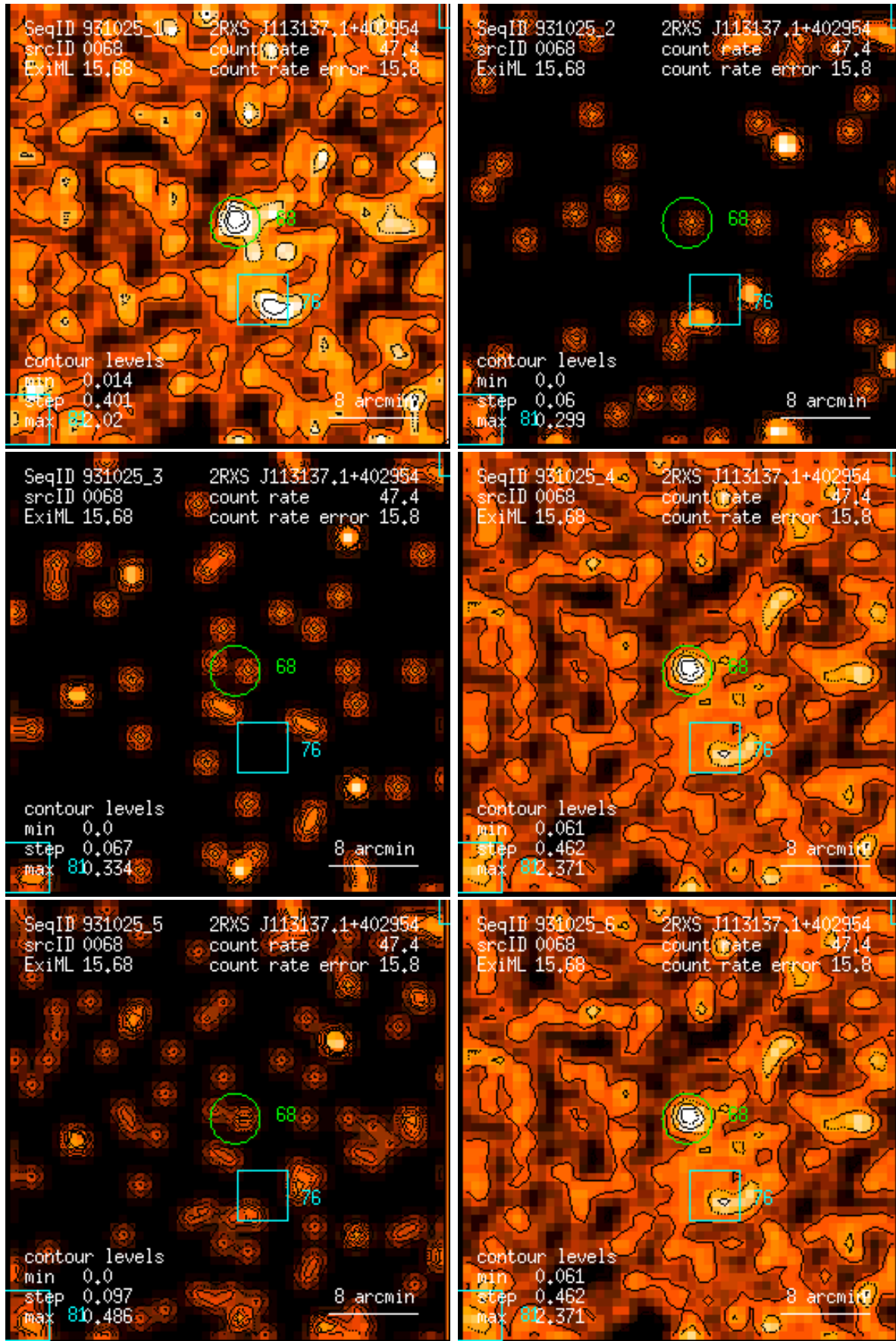
Figure 68: RASS 931025: detection 0068: band rate images, Gaussian filter: (1) PSPC channels 11 – 41, (2) 52 – 90, (3) 91 – 201, (4) 11 – 235, (5) 52 – 201, (6) 11 – 201. Broad band rates in counts/ks. Band rate contour levels in counts/ks/arcmin 2 .
