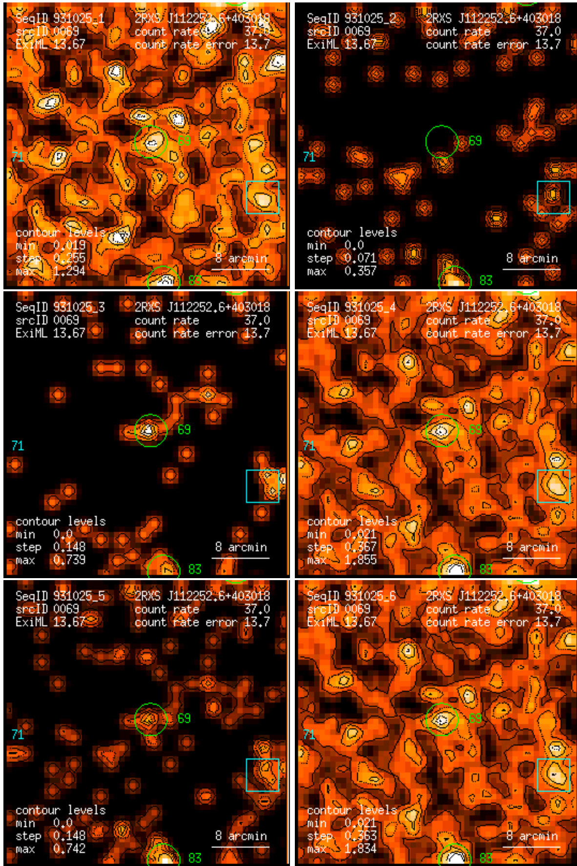
Figure 69: RASS 931025: detection 0069: band rate images, Gaussian filter: (1) PSPC channels 11 – 41, (2) 52 – 90, (3) 91 – 201, (4) 11 – 235, (5) 52 – 201, (6) 11 – 201. Broad band rates in counts/ks. Band rate contour levels in counts/ks/arcmin 2 .
