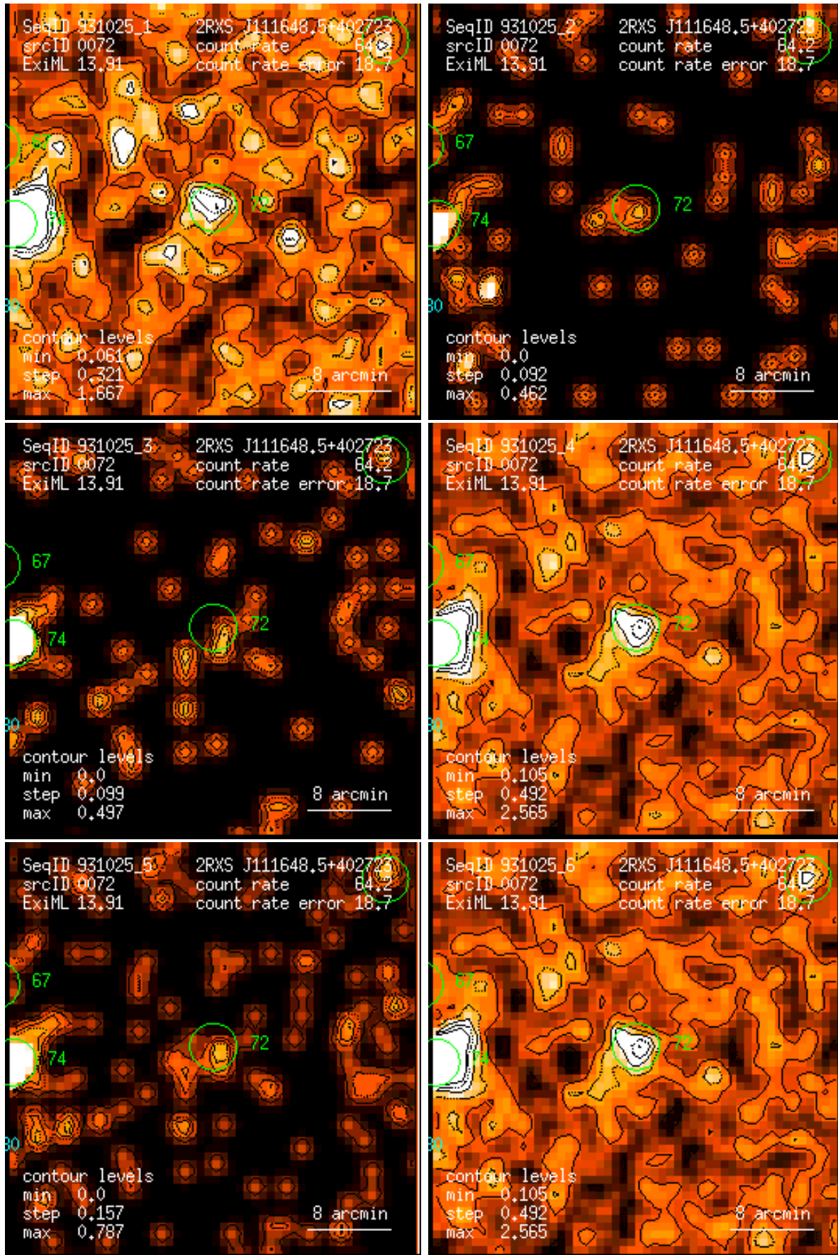
Figure 72: RASS 931025: detection 0072: band rate images, Gaussian filter: (1) PSPC channels 11 – 41, (2) 52 – 90, (3) 91 – 201, (4) 11 – 235, (5) 52 – 201, (6) 11 – 201. Broad band rates in counts/ks. Band rate contour levels in counts/ks/arcmin 2 .
