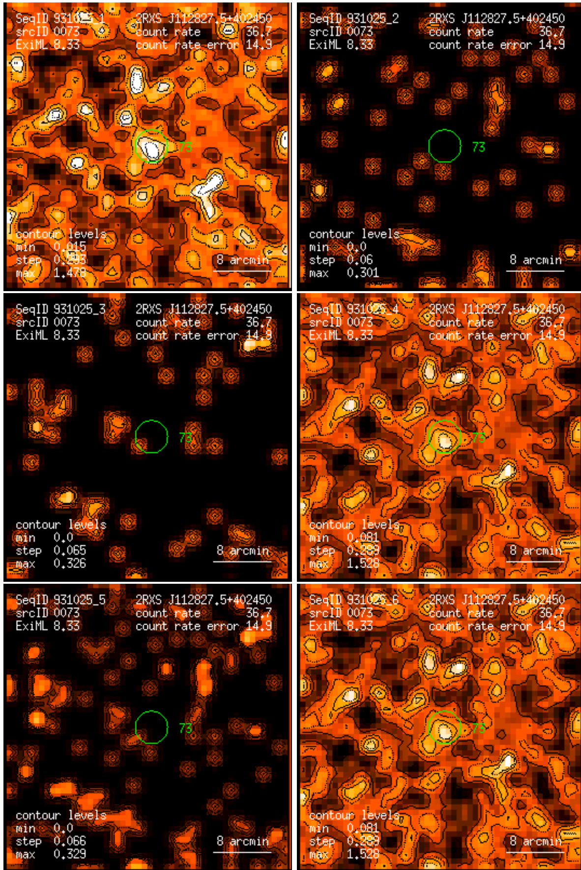
Figure 73: RASS 931025: detection 0073: band rate images, Gaussian filter: (1) PSPC channels 11 – 41, (2) 52 – 90, (3) 91 – 201, (4) 11 – 235, (5) 52 – 201, (6) 11 – 201. Broad band rates in counts/ks. Band rate contour levels in counts/ks/arcmin 2 .
