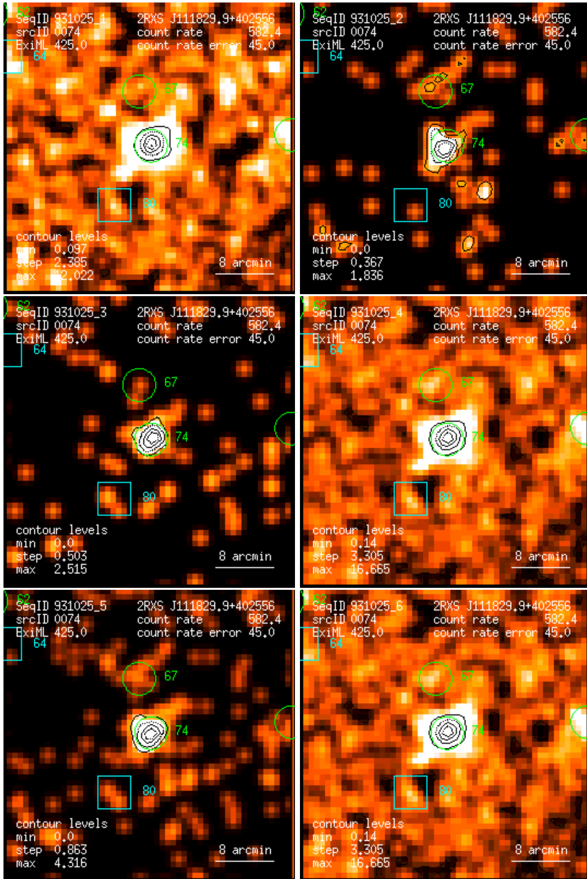
Figure 74: RASS 931025: detection 0074: band rate images, Gaussian filter: (1) PSPC channels 11 – 41, (2) 52 – 90, (3) 91 – 201, (4) 11 – 235, (5) 52 – 201, (6) 11 – 201. Broad band rates in counts/ks. Band rate contour levels in counts/ks/arcmin 2 .
