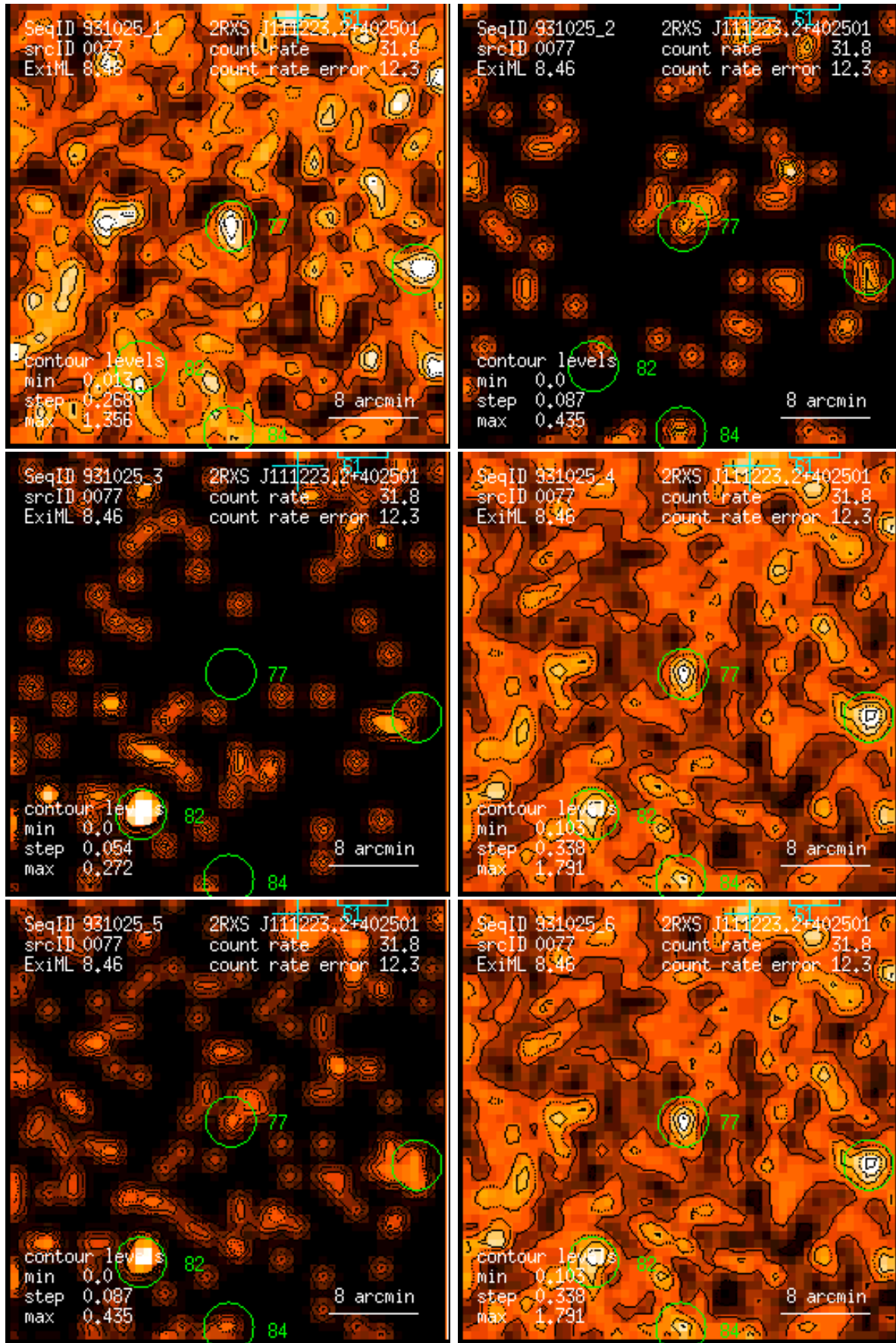
Figure 77: RASS 931025: detection 0077: band rate images, Gaussian filter: (1) PSPC channels 11 – 41, (2) 52 – 90, (3) 91 – 201, (4) 11 – 235, (5) 52 – 201, (6) 11 – 201. Broad band rates in counts/ks. Band rate contour levels in counts/ks/arcmin 2 .
