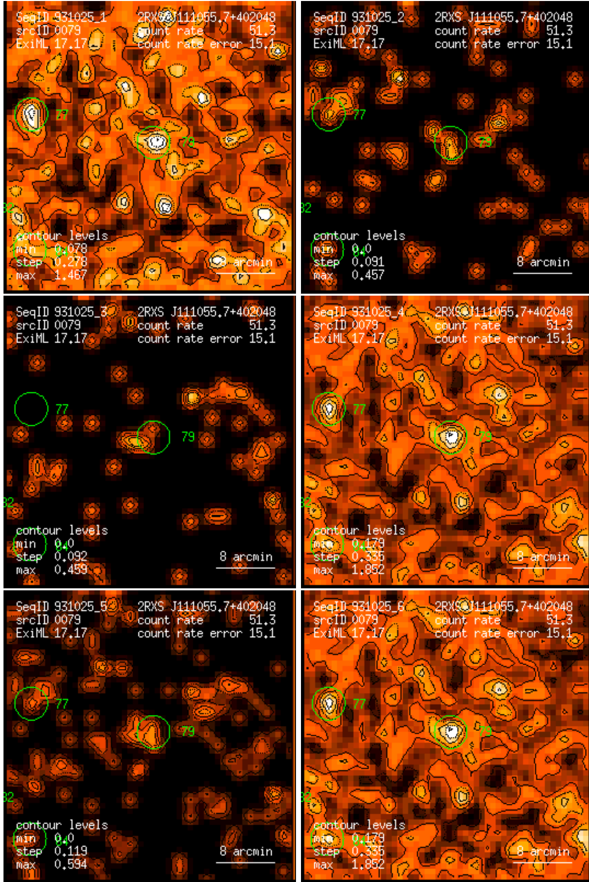
Figure 79: RASS 931025: detection 0079: band rate images, Gaussian filter: (1) PSPC channels 11 – 41, (2) 52 – 90, (3) 91 – 201, (4) 11 – 235, (5) 52 – 201, (6) 11 – 201. Broad band rates in counts/ks. Band rate contour levels in counts/ks/arcmin 2 .
