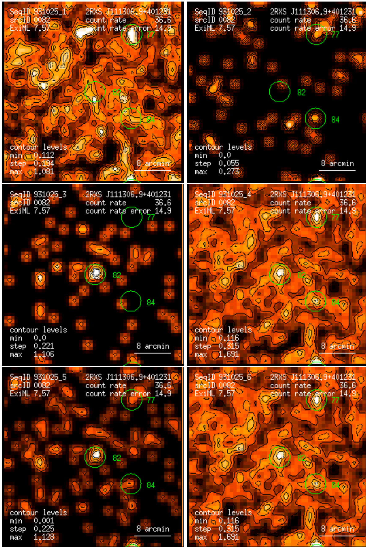
Figure 82: RASS 931025: detection 0082: band rate images, Gaussian filter: (1) PSPC channels 11 – 41, (2) 52 – 90, (3) 91 – 201, (4) 11 – 235, (5) 52 – 201, (6) 11 – 201. Broad band rates in counts/ks. Band rate contour levels in counts/ks/arcmin 2 .
