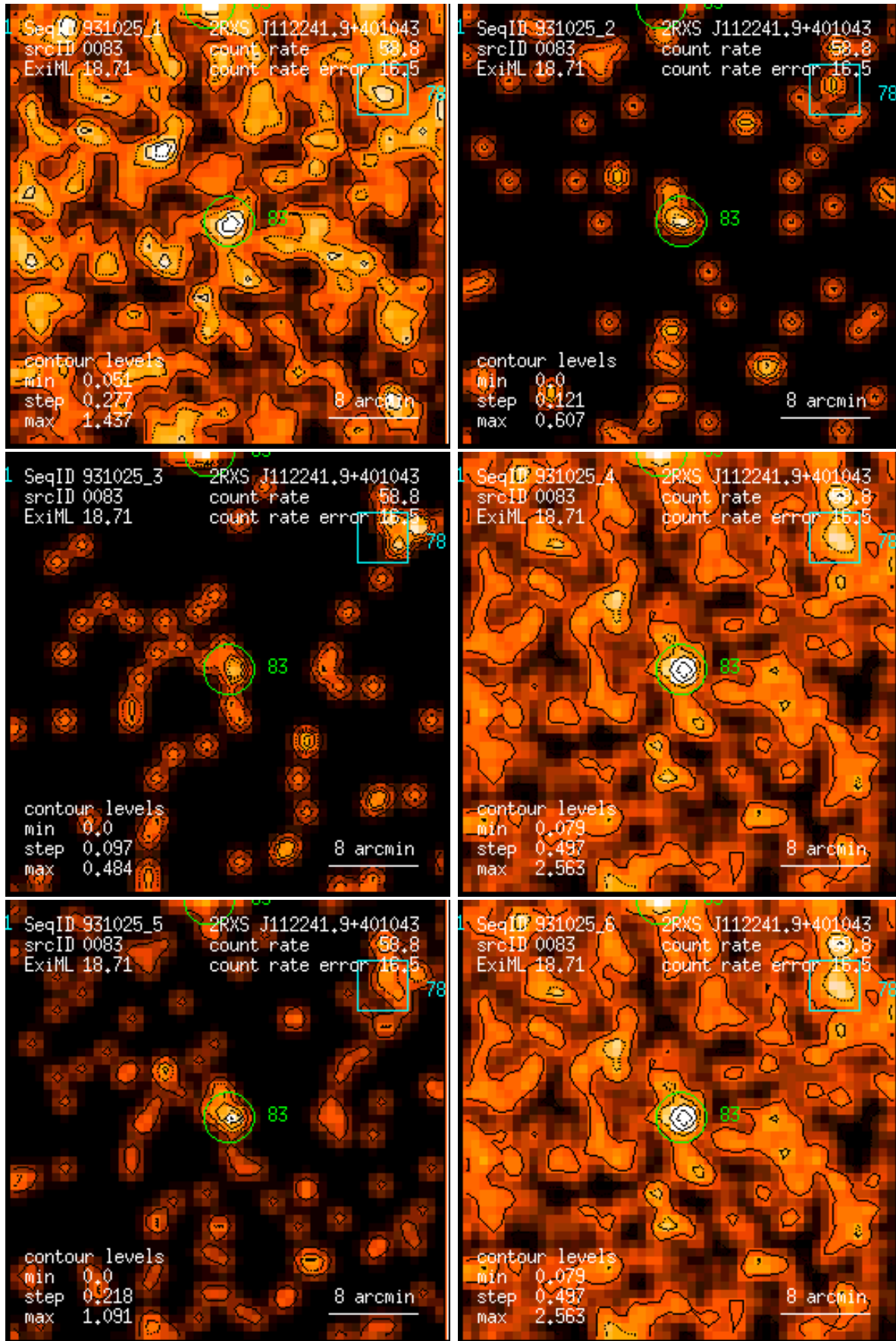
Figure 83: RASS 931025: detection 0083: band rate images, Gaussian filter: (1) PSPC channels 11 – 41, (2) 52 – 90, (3) 91 – 201, (4) 11 – 235, (5) 52 – 201, (6) 11 – 201. Broad band rates in counts/ks. Band rate contour levels in counts/ks/arcmin 2 .
