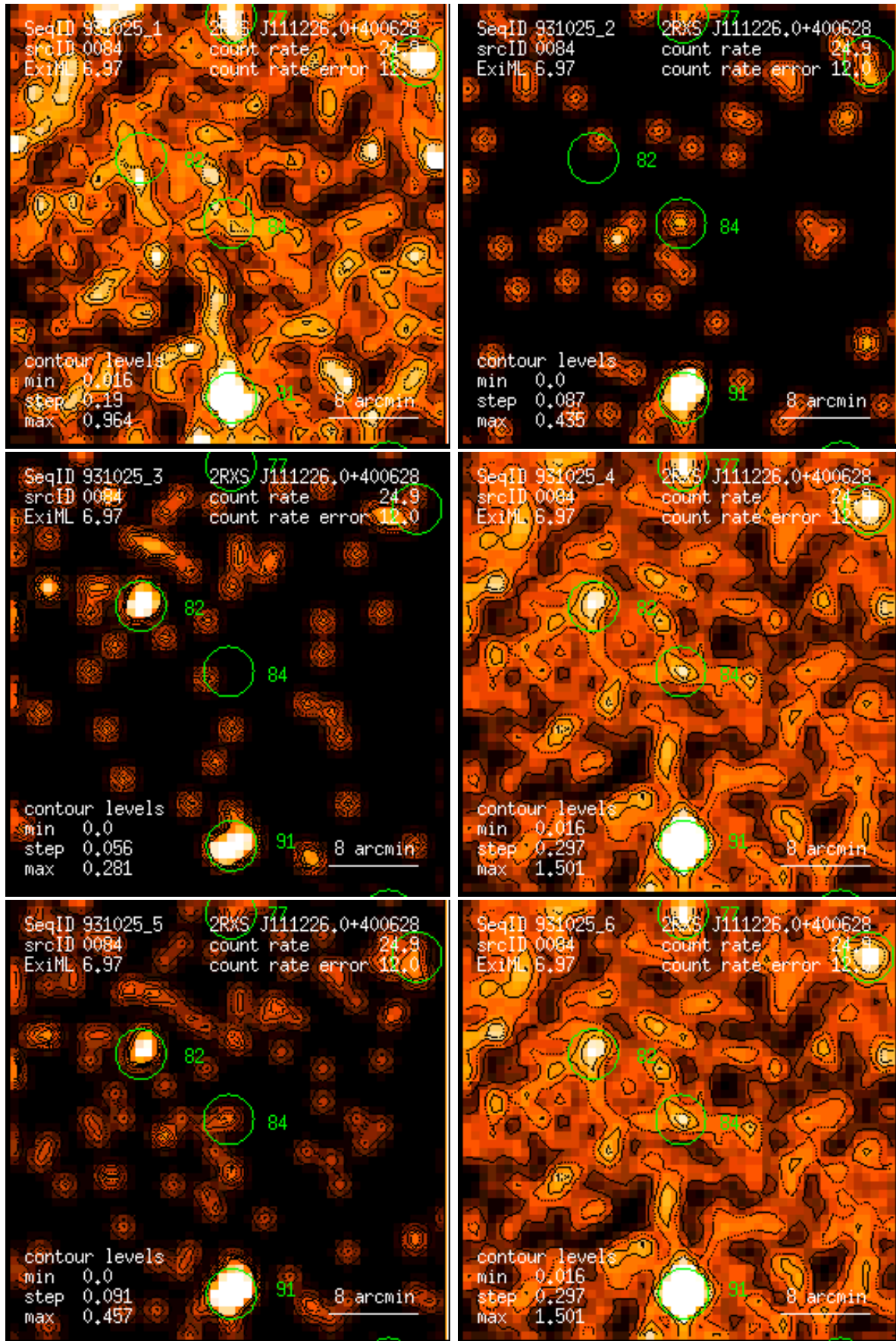
Figure 84: RASS 931025: detection 0084: band rate images, Gaussian filter: (1) PSPC channels 11 – 41, (2) 52 – 90, (3) 91 – 201, (4) 11 – 235, (5) 52 – 201, (6) 11 – 201. Broad band rates in counts/ks. Band rate contour levels in counts/ks/arcmin 2 .
