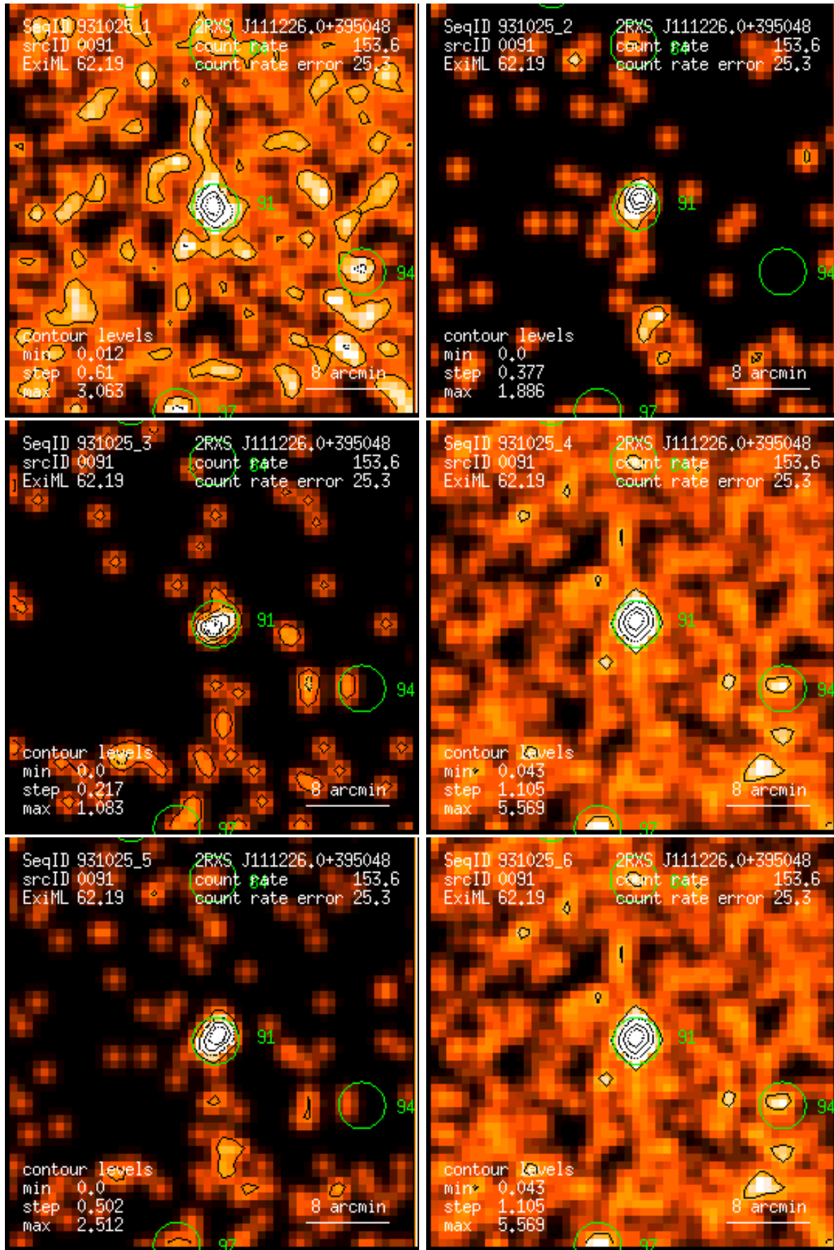
Figure 91: RASS 931025: detection 0091: band rate images, Gaussian filter: (1) PSPC channels 11 – 41, (2) 52 – 90, (3) 91 – 201, (4) 11 – 235, (5) 52 – 201, (6) 11 – 201. Broad band rates in counts/ks. Band rate contour levels in counts/ks/arcmin 2 .
