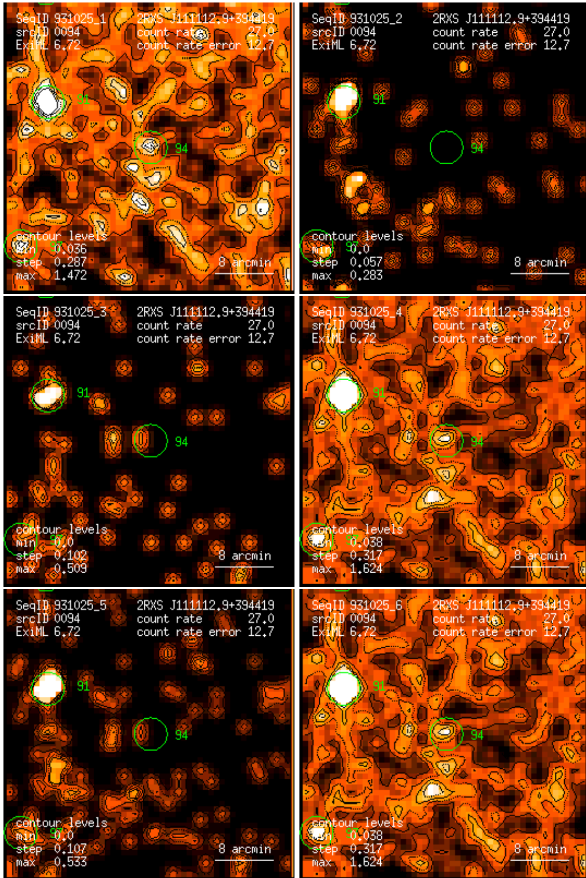
Figure 94: RASS 931025: detection 0094: band rate images, Gaussian filter: (1) PSPC channels 11 – 41, (2) 52 – 90, (3) 91 – 201, (4) 11 – 235, (5) 52 – 201, (6) 11 – 201. Broad band rates in counts/ks. Band rate contour levels in counts/ks/arcmin 2 .
