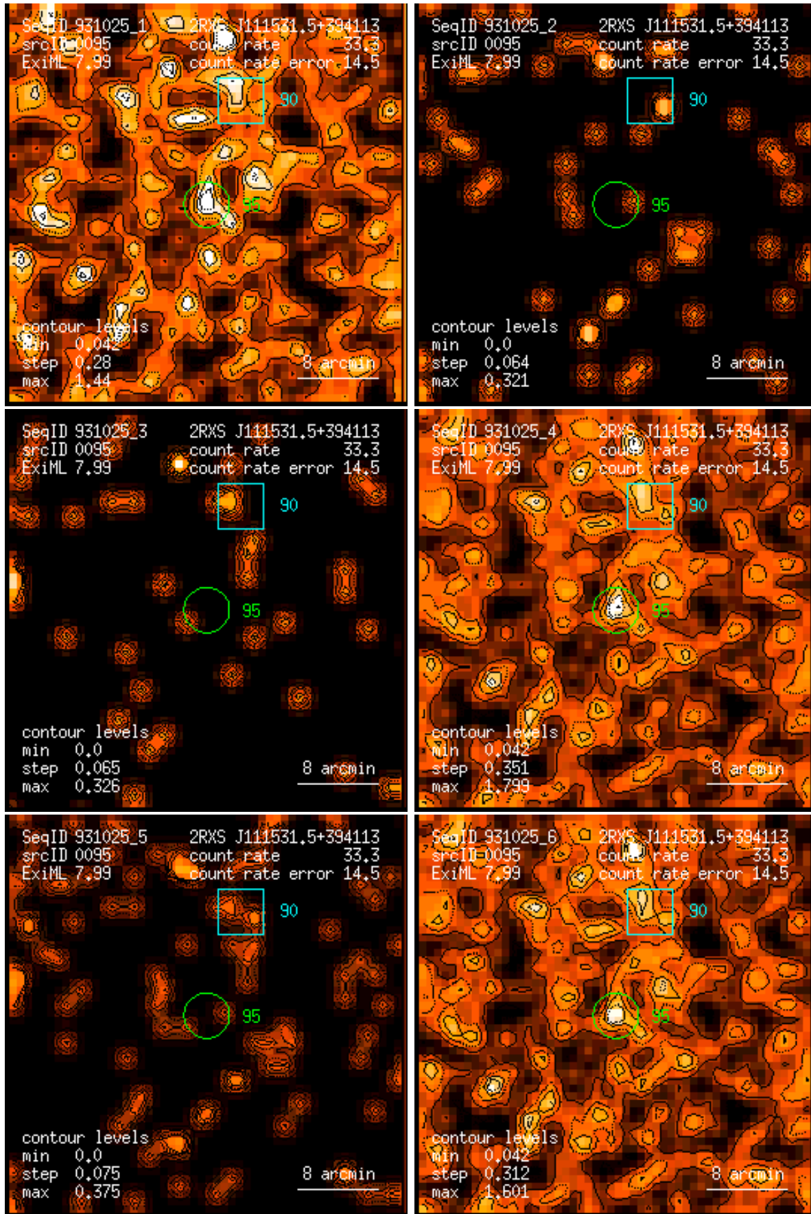
Figure 95: RASS 931025: detection 0095: band rate images, Gaussian filter: (1) PSPC channels 11 – 41, (2) 52 – 90, (3) 91 – 201, (4) 11 – 235, (5) 52 – 201, (6) 11 – 201. Broad band rates in counts/ks. Band rate contour levels in counts/ks/arcmin 2 .
