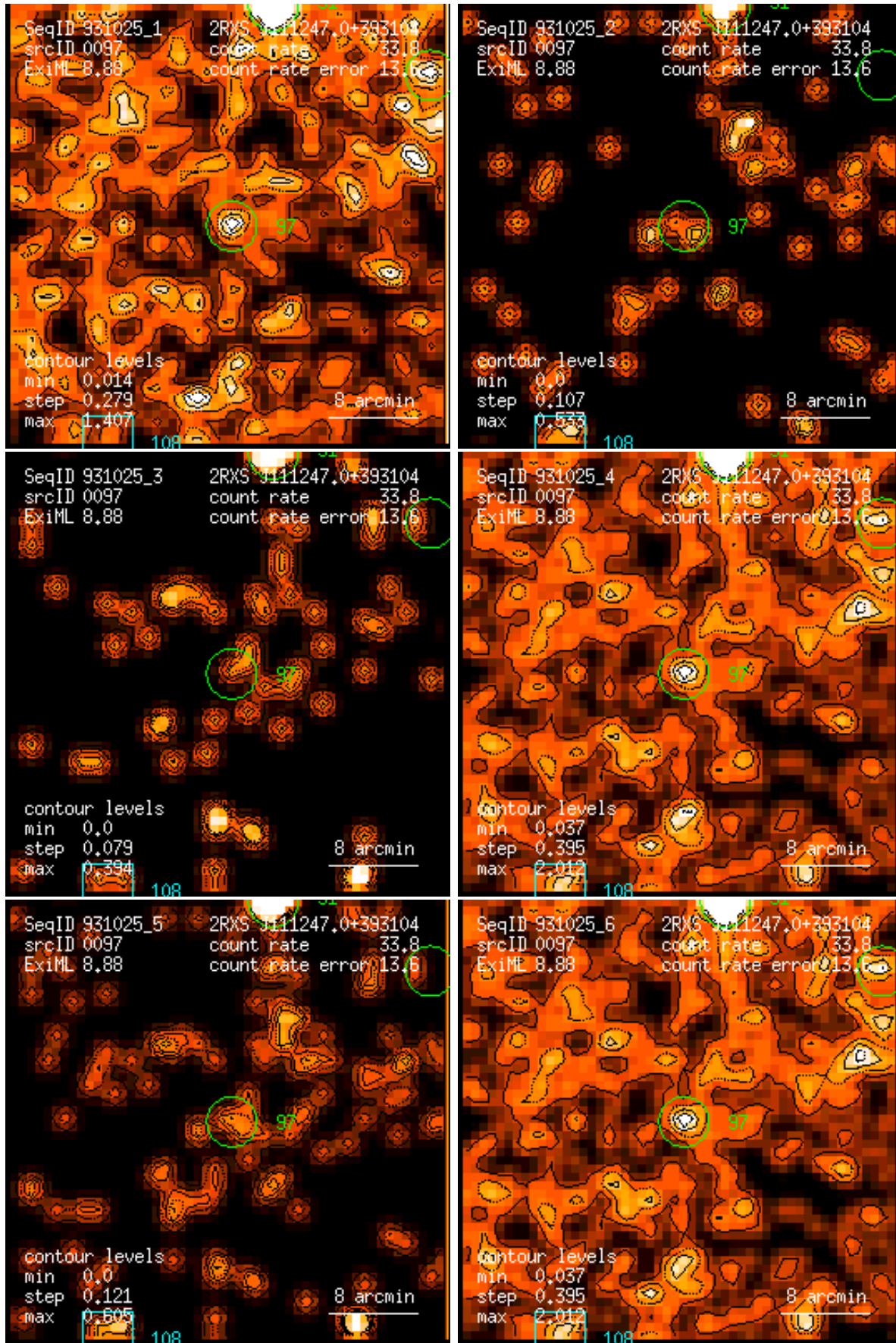
Figure 97: RASS 931025: detection 0097: band rate images, Gaussian filter: (1) PSPC channels 11 – 41, (2) 52 – 90, (3) 91 – 201, (4) 11 – 235, (5) 52 – 201, (6) 11 – 201. Broad band rates in counts/ks. Band rate contour levels in counts/ks/arcmin 2 .
