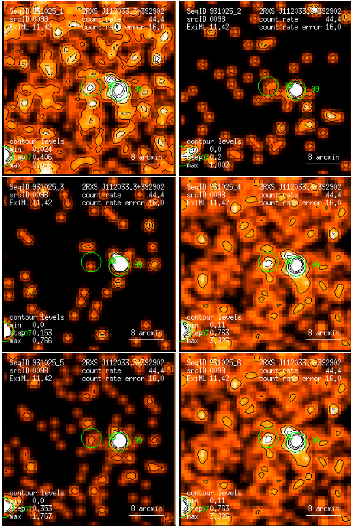
Figure 98: RASS 931025: detection 0098: band rate images, Gaussian filter: (1) PSPC channels 11 – 41, (2) 52 – 90, (3) 91 – 201, (4) 11 – 235, (5) 52 – 201, (6) 11 – 201. Broad band rates in counts/ks. Band rate contour levels in counts/ks/arcmin 2 .
