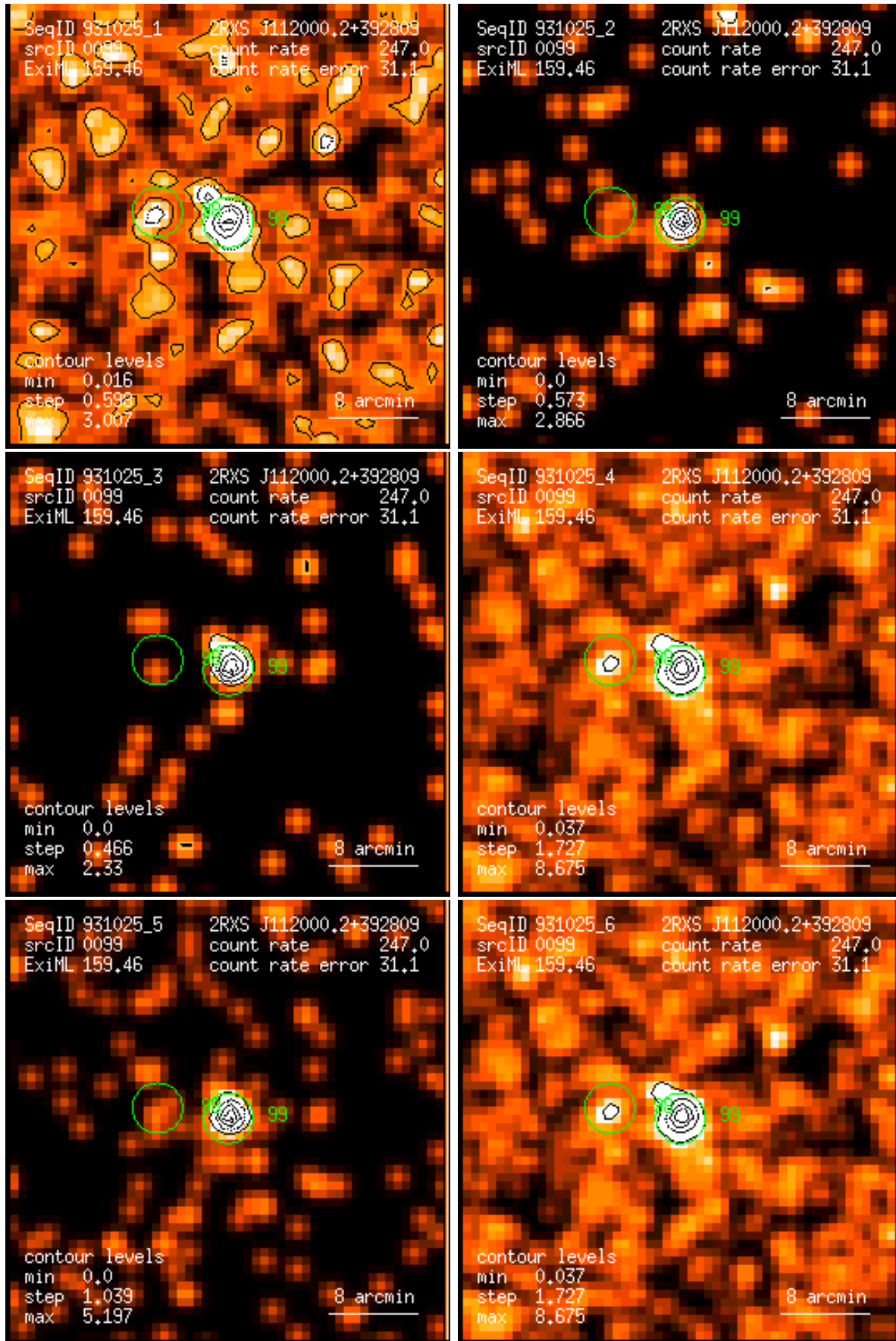
Figure 99: RASS 931025: detection 0099: band rate images, Gaussian filter: (1) PSPC channels 11 – 41, (2) 52 – 90, (3) 91 – 201, (4) 11 – 235, (5) 52 – 201, (6) 11 – 201. Broad band rates in counts/ks. Band rate contour levels in counts/ks/arcmin 2 .
