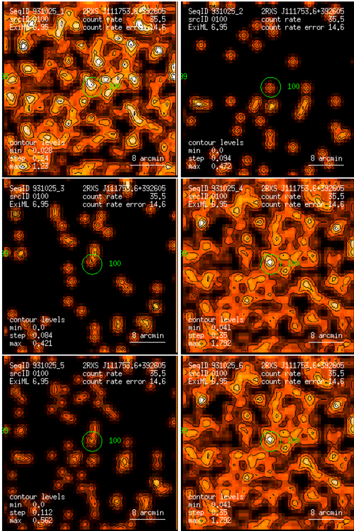
Figure 100: RASS 931025: detection 0100: band rate images, Gaussian filter: (1) PSPC channels 11 – 41, (2) 52 – 90, (3) 91 – 201, (4) 11 – 235, (5) 52 – 201, (6) 11 – 201. Broad band rates in counts/ks. Band rate contour levels in counts/ks/arcmin 2 .
