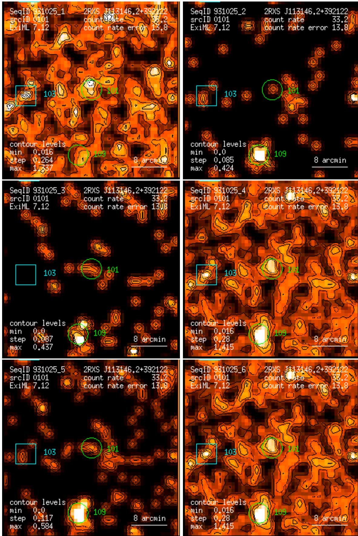
Figure 101: RASS 931025: detection 0101: band rate images, Gaussian filter: (1) PSPC channels 11 – 41, (2) 52 – 90, (3) 91 – 201, (4) 11 – 235, (5) 52 – 201, (6) 11 – 201. Broad band rates in counts/ks. Band rate contour levels in counts/ks/arcmin 2 .
