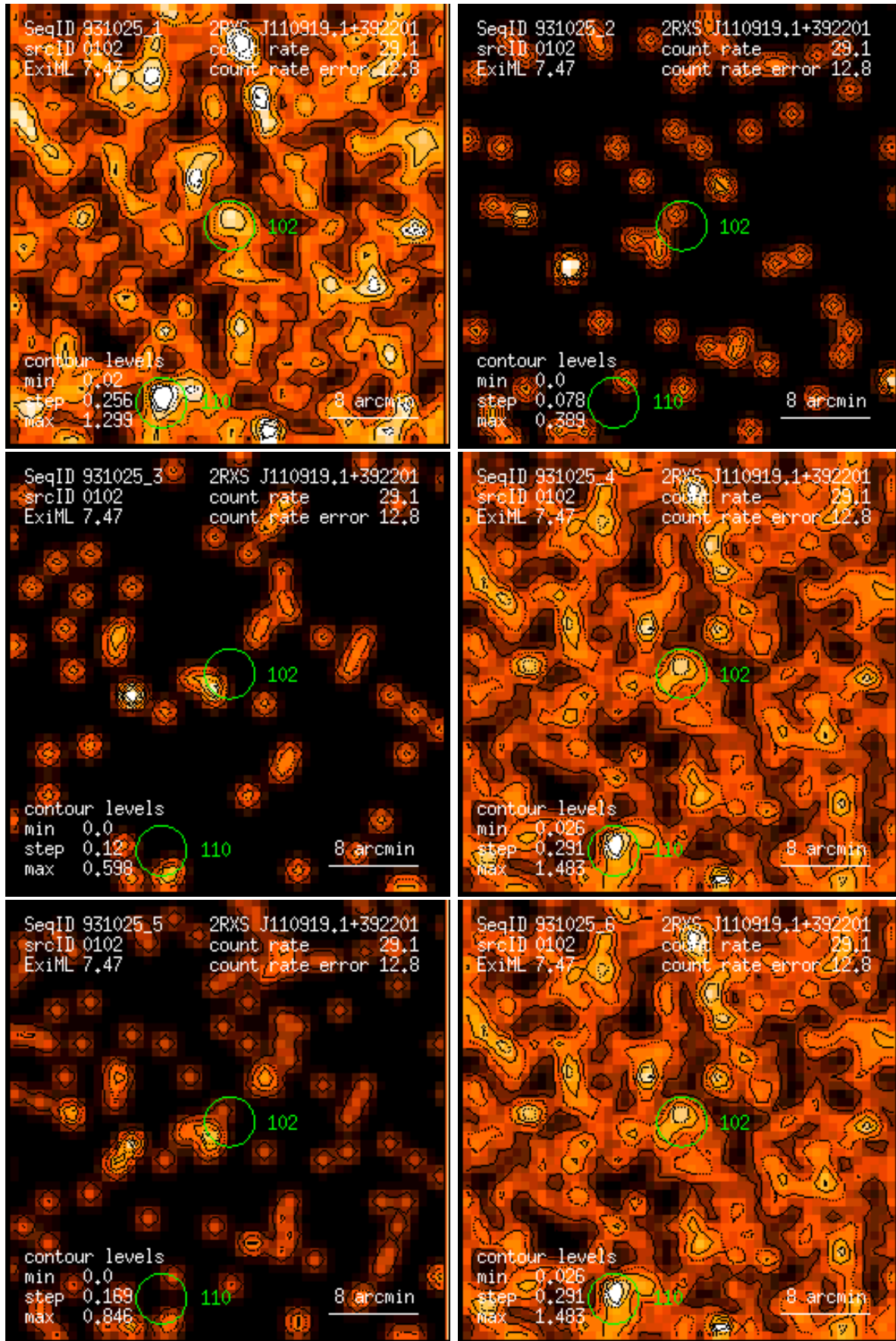
Figure 102: RASS 931025: detection 0102: band rate images, Gaussian filter: (1) PSPC channels 11 – 41, (2) 52 – 90, (3) 91 – 201, (4) 11 – 235, (5) 52 – 201, (6) 11 – 201. Broad band rates in counts/ks. Band rate contour levels in counts/ks/arcmin 2 .
