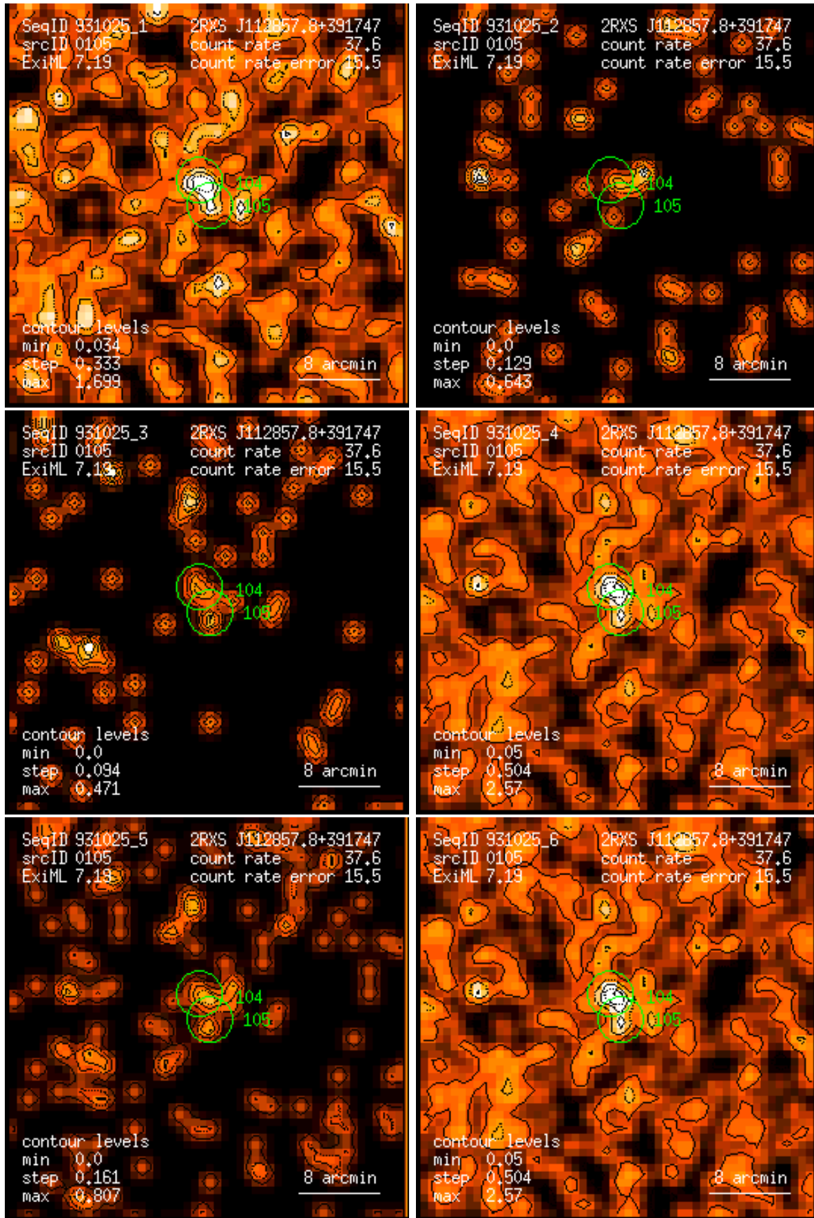
Figure 105: RASS 931025: detection 0105: band rate images, Gaussian filter: (1) PSPC channels 11 – 41, (2) 52 – 90, (3) 91 – 201, (4) 11 – 235, (5) 52 – 201, (6) 11 – 201. Broad band rates in counts/ks. Band rate contour levels in counts/ks/arcmin 2 .
