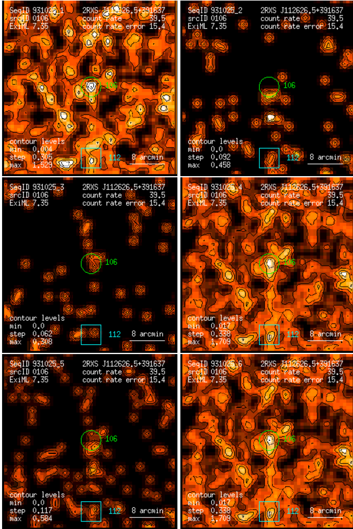
Figure 106: RASS 931025: detection 0106: band rate images, Gaussian filter: (1) PSPC channels 11 – 41, (2) 52 – 90, (3) 91 – 201, (4) 11 – 235, (5) 52 – 201, (6) 11 – 201. Broad band rates in counts/ks. Band rate contour levels in counts/ks/arcmin 2 .
