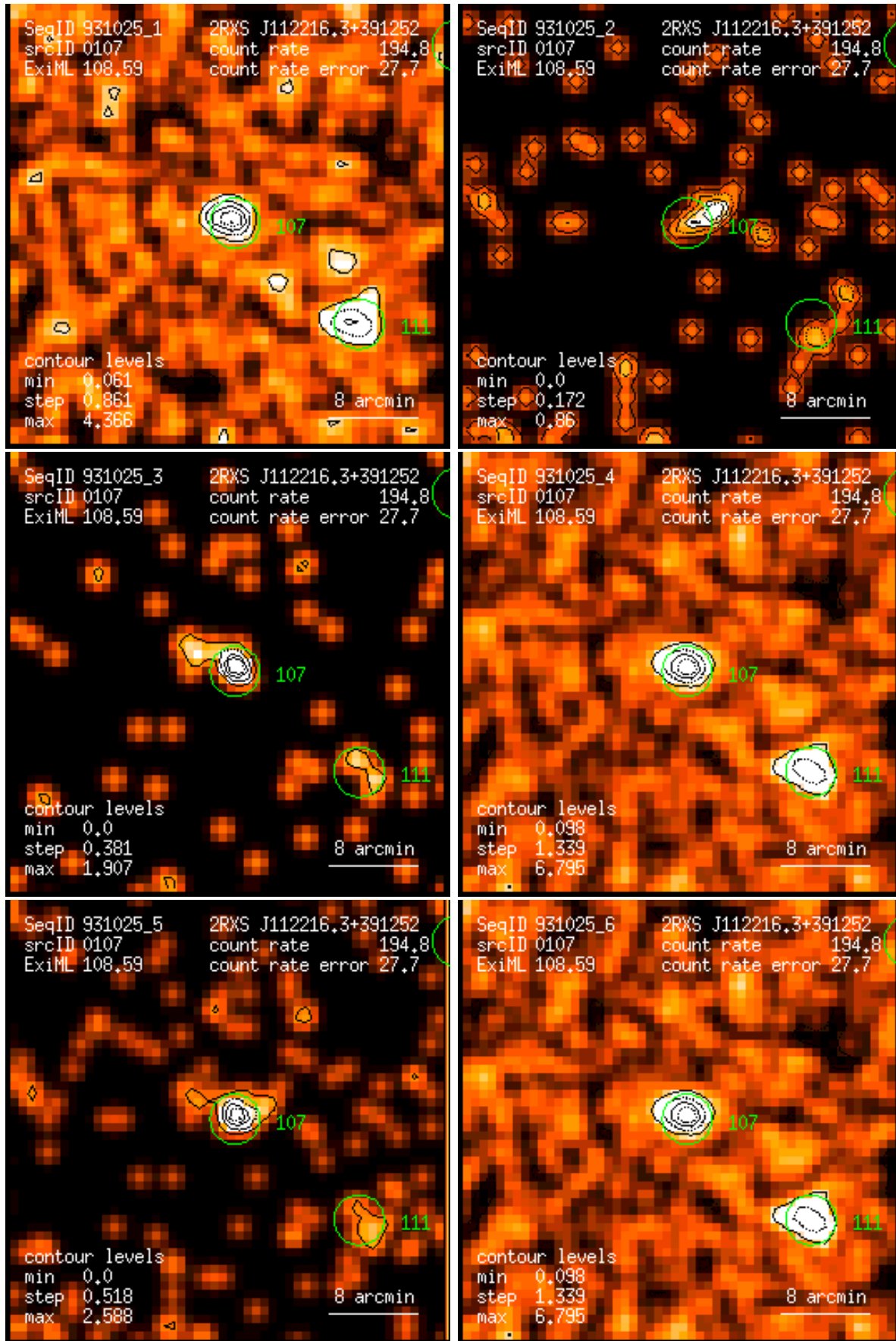
Figure 107: RASS 931025: detection 0107: band rate images, Gaussian filter: (1) PSPC channels 11 – 41, (2) 52 – 90, (3) 91 – 201, (4) 11 – 235, (5) 52 – 201, (6) 11 – 201. Broad band rates in counts/ks. Band rate contour levels in counts/ks/arcmin 2 .
