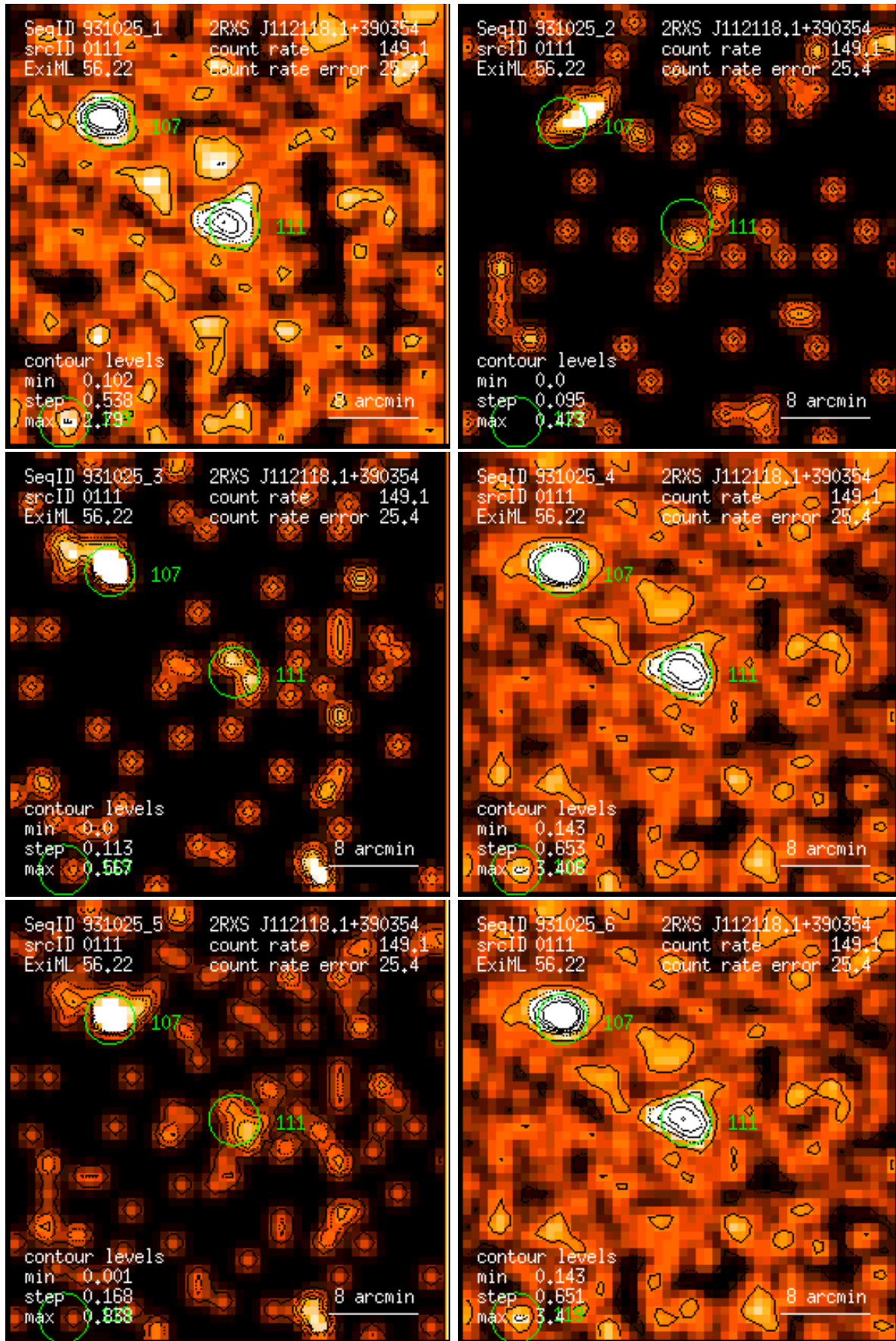
Figure 111: RASS 931025: detection 0111: band rate images, Gaussian filter: (1) PSPC channels 11 – 41, (2) 52 – 90, (3) 91 – 201, (4) 11 – 235, (5) 52 – 201, (6) 11 – 201. Broad band rates in counts/ks. Band rate contour levels in counts/ks/arcmin 2 .
