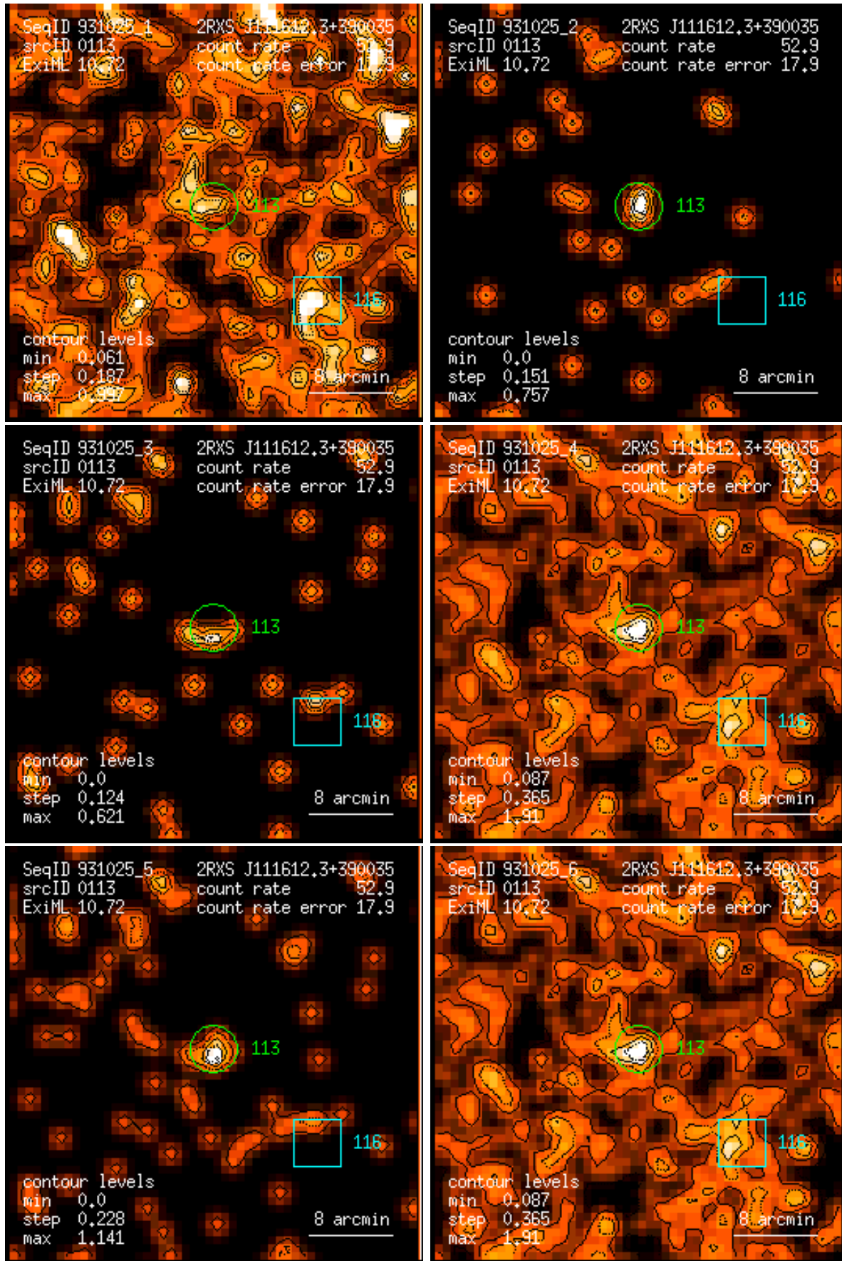
Figure 113: RASS 931025: detection 0113: band rate images, Gaussian filter: (1) PSPC channels 11 – 41, (2) 52 – 90, (3) 91 – 201, (4) 11 – 235, (5) 52 – 201, (6) 11 – 201. Broad band rates in counts/ks. Band rate contour levels in counts/ks/arcmin 2 .
