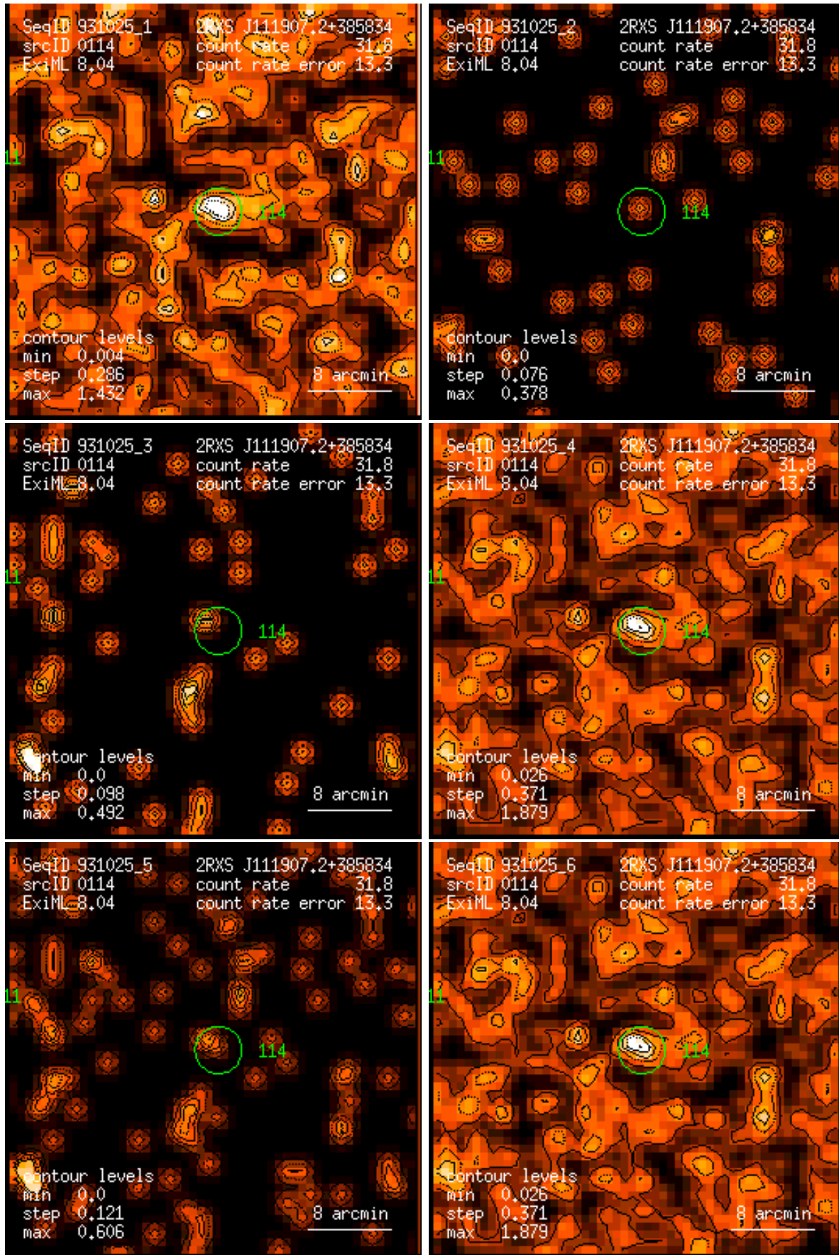
Figure 114: RASS 931025: detection 0114: band rate images, Gaussian filter: (1) PSPC channels 11 – 41, (2) 52 – 90, (3) 91 – 201, (4) 11 – 235, (5) 52 – 201, (6) 11 – 201. Broad band rates in counts/ks. Band rate contour levels in counts/ks/arcmin 2 .
