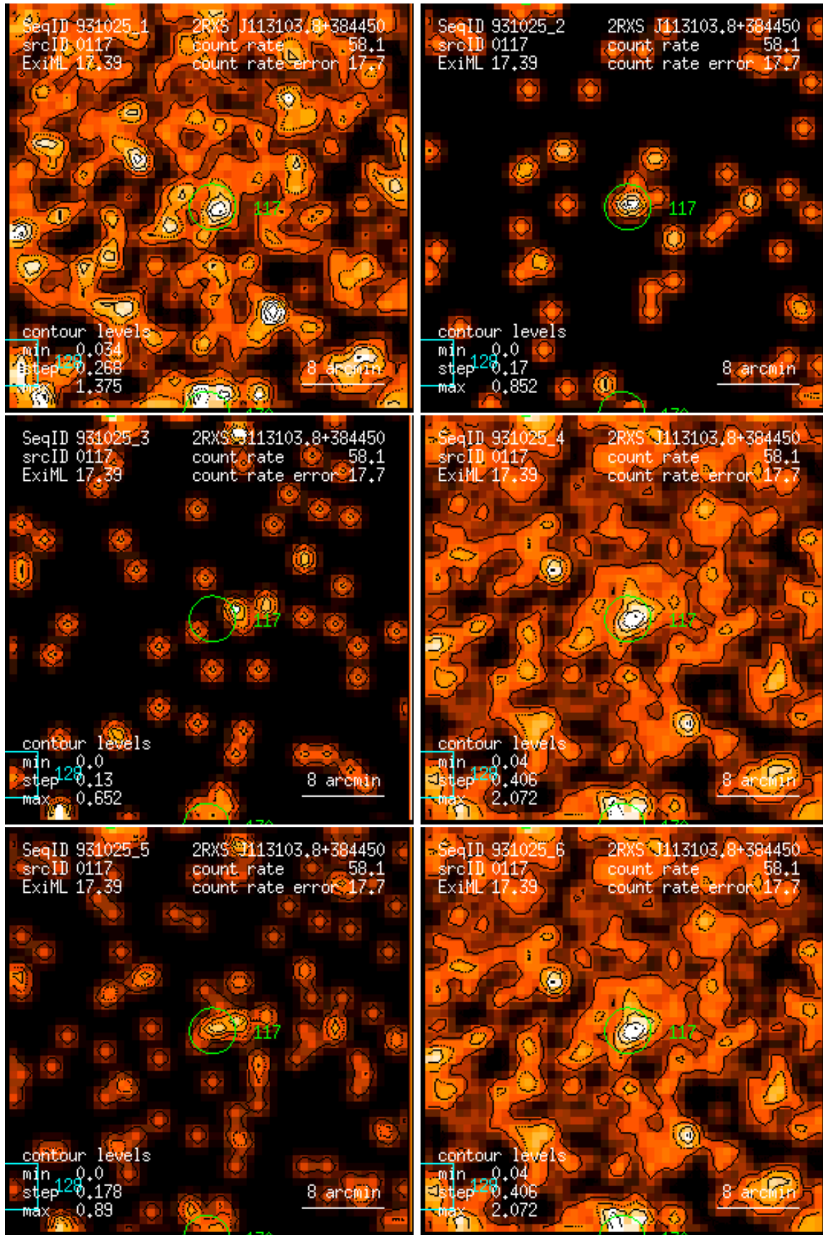
Figure 117: RASS 931025: detection 0117: band rate images, Gaussian filter: (1) PSPC channels 11 – 41, (2) 52 – 90, (3) 91 – 201, (4) 11 – 235, (5) 52 – 201, (6) 11 – 201. Broad band rates in counts/ks. Band rate contour levels in counts/ks/arcmin 2 .
