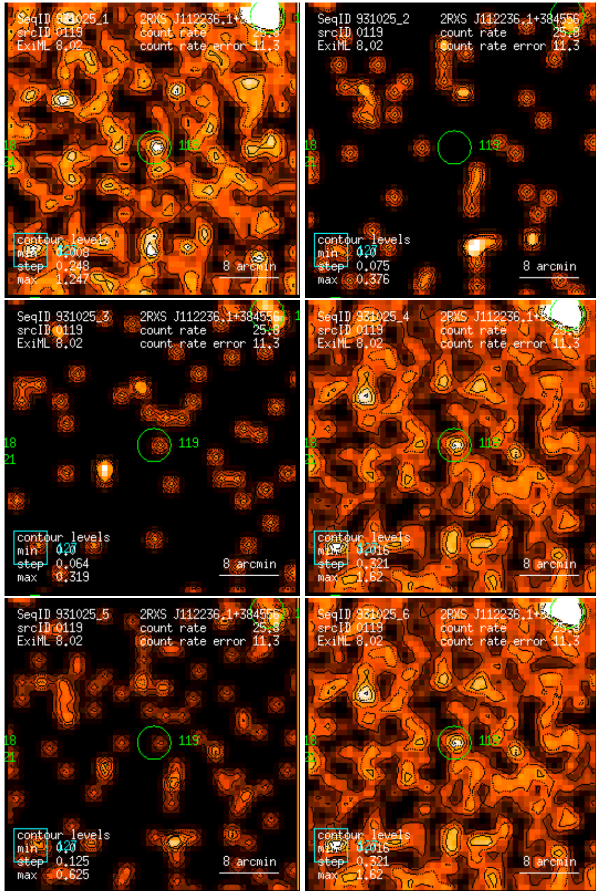
Figure 119: RASS 931025: detection 0119: band rate images, Gaussian filter: (1) PSPC channels 11 – 41, (2) 52 – 90, (3) 91 – 201, (4) 11 – 235, (5) 52 – 201, (6) 11 – 201. Broad band rates in counts/ks. Band rate contour levels in counts/ks/arcmin 2 .
