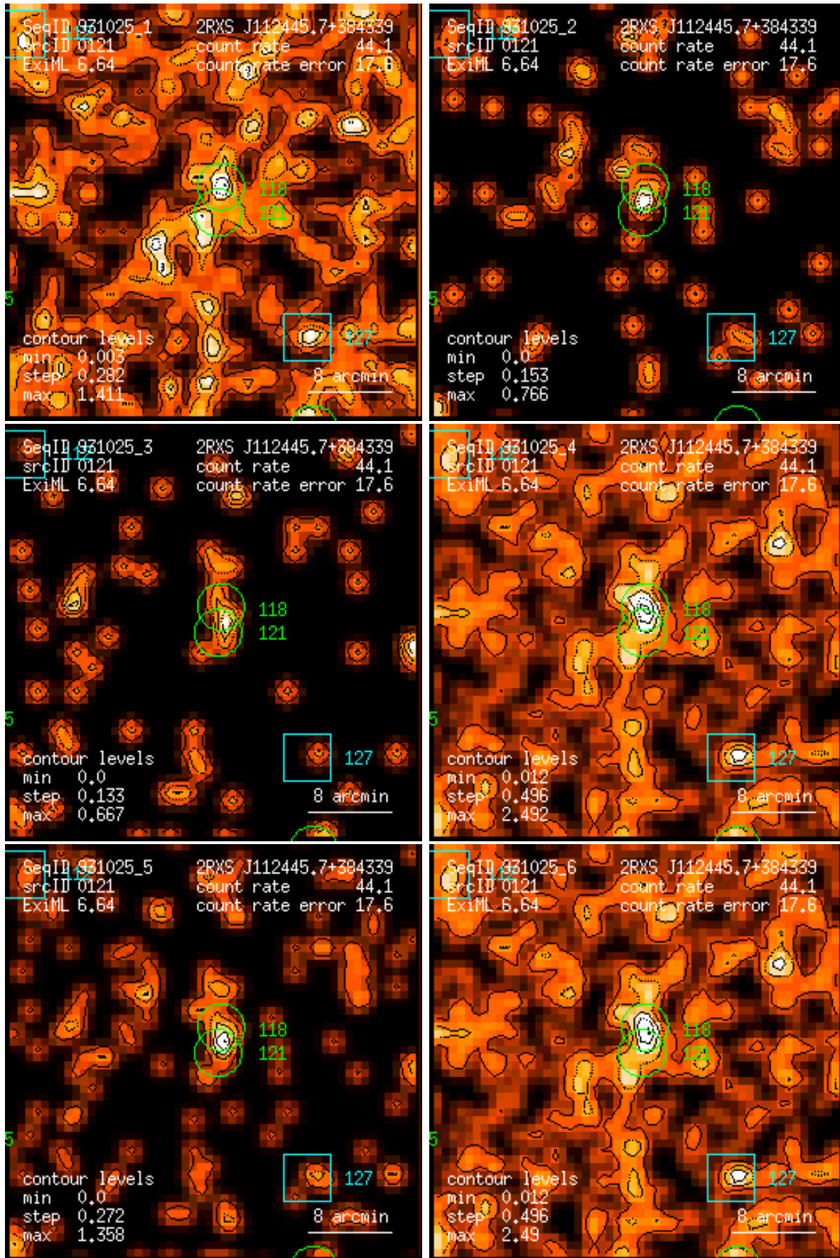
Figure 121: RASS 931025: detection 0121: band rate images, Gaussian filter: (1) PSPC channels 11 – 41, (2) 52 – 90, (3) 91 – 201, (4) 11 – 235, (5) 52 – 201, (6) 11 – 201. Broad band rates in counts/ks. Band rate contour levels in counts/ks/arcmin 2 .
