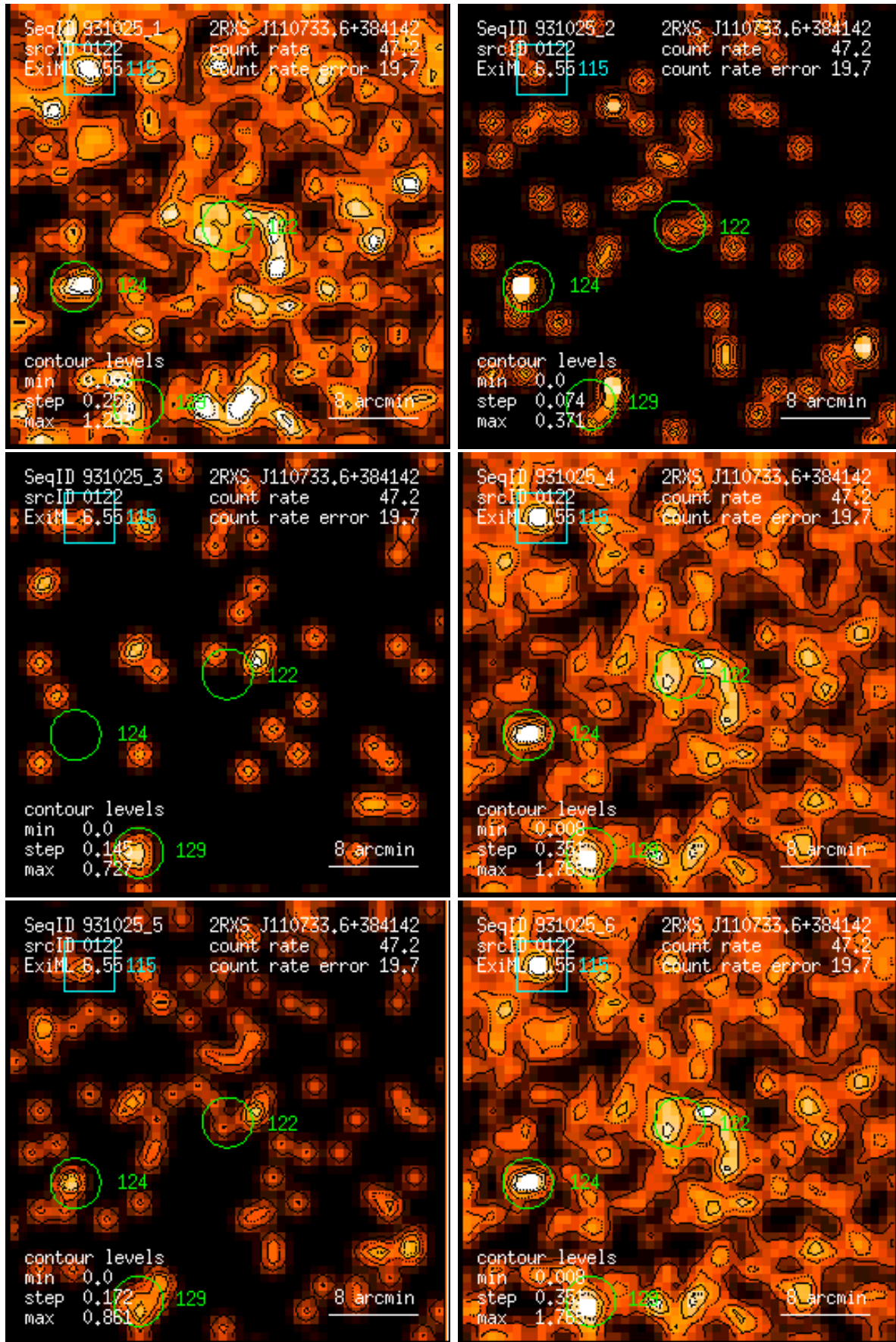
Figure 122: RASS 931025: detection 0122: band rate images, Gaussian filter: (1) PSPC channels 11 – 41, (2) 52 – 90, (3) 91 – 201, (4) 11 – 235, (5) 52 – 201, (6) 11 – 201. Broad band rates in counts/ks. Band rate contour levels in counts/ks/arcmin 2 .
