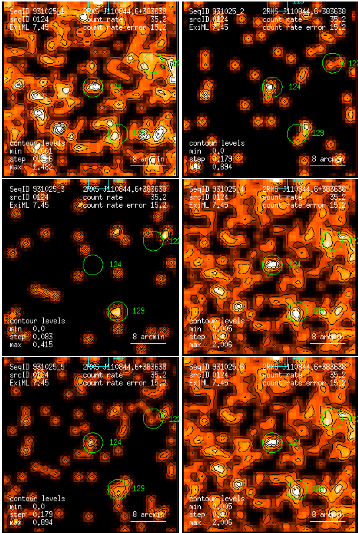
Figure 124: RASS 931025: detection 0124: band rate images, Gaussian filter: (1) PSPC channels 11 – 41, (2) 52 – 90, (3) 91 – 201, (4) 11 – 235, (5) 52 – 201, (6) 11 – 201. Broad band rates in counts/ks. Band rate contour levels in counts/ks/arcmin 2 .
