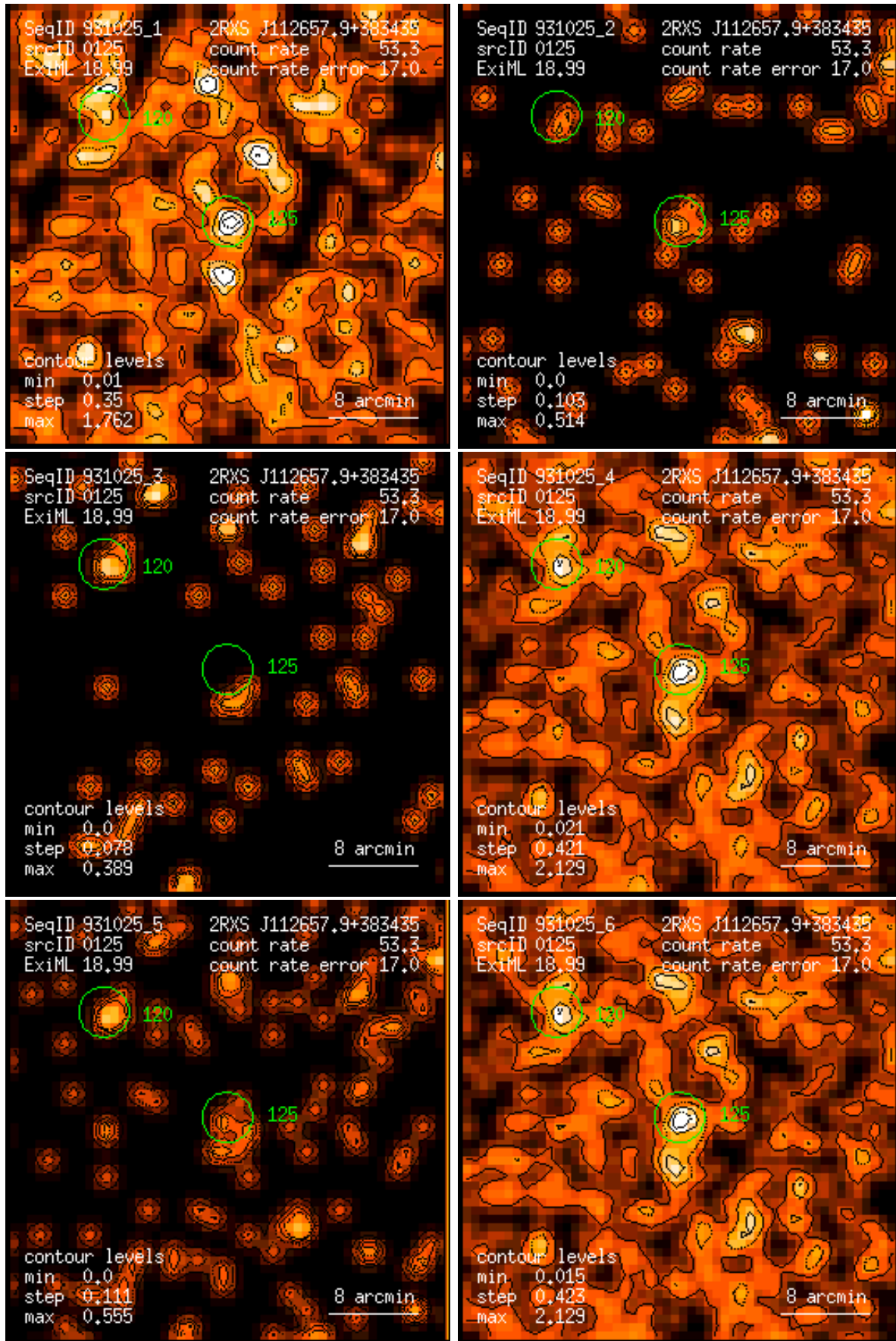
Figure 125: RASS 931025: detection 0125: band rate images, Gaussian filter: (1) PSPC channels 11 – 41, (2) 52 – 90, (3) 91 – 201, (4) 11 – 235, (5) 52 – 201, (6) 11 – 201. Broad band rates in counts/ks. Band rate contour levels in counts/ks/arcmin 2 .
