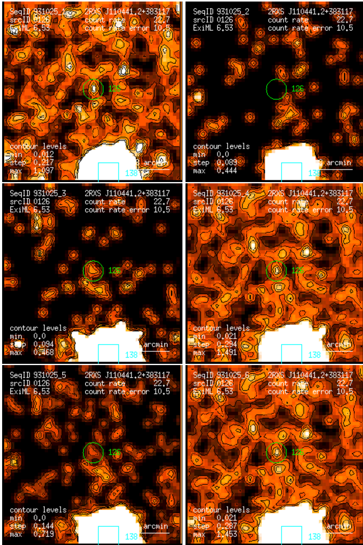
Figure 126: RASS 931025: detection 0126: band rate images, Gaussian filter: (1) PSPC channels 11 – 41, (2) 52 – 90, (3) 91 – 201, (4) 11 – 235, (5) 52 – 201, (6) 11 – 201. Broad band rates in counts/ks. Band rate contour levels in counts/ks/arcmin 2 .
