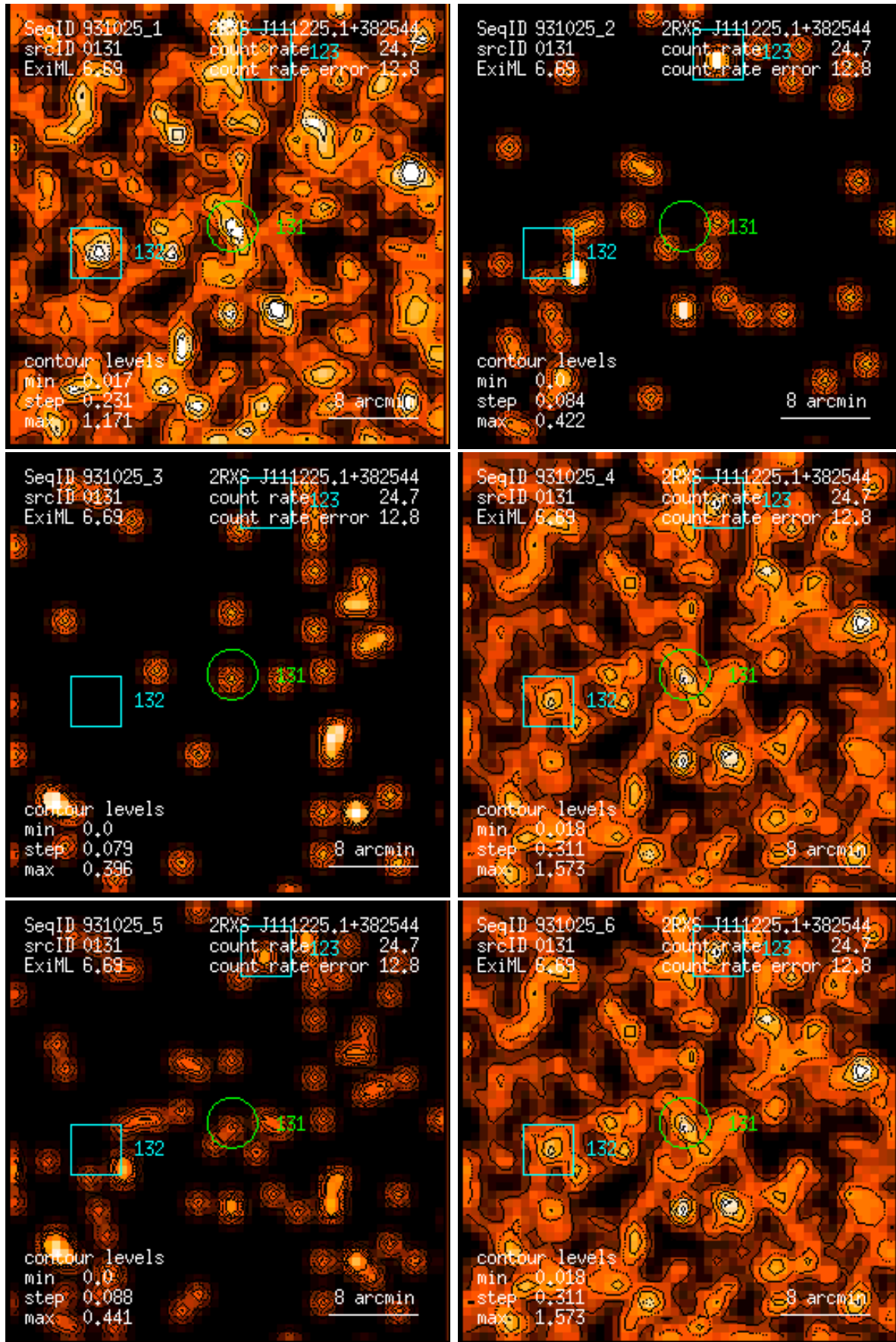
Figure 131: RASS 931025: detection 0131: band rate images, Gaussian filter: (1) PSPC channels 11 – 41, (2) 52 – 90, (3) 91 – 201, (4) 11 – 235, (5) 52 – 201, (6) 11 – 201. Broad band rates in counts/ks. Band rate contour levels in counts/ks/arcmin 2 .
