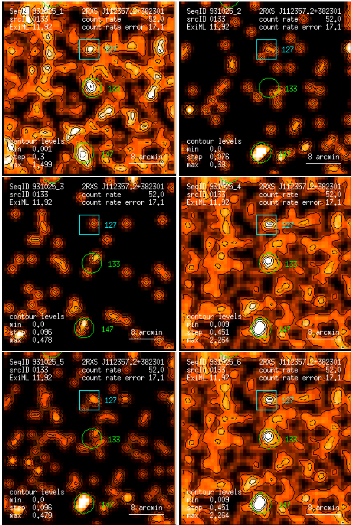
Figure 133: RASS 931025: detection 0133: band rate images, Gaussian filter: (1) PSPC channels 11 – 41, (2) 52 – 90, (3) 91 – 201, (4) 11 – 235, (5) 52 – 201, (6) 11 – 201. Broad band rates in counts/ks. Band rate contour levels in counts/ks/arcmin 2 .
