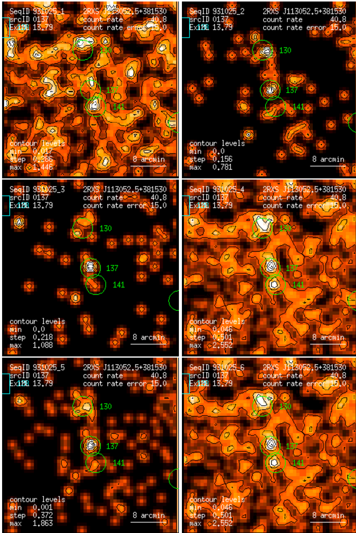
Figure 137: RASS 931025: detection 0137: band rate images, Gaussian filter: (1) PSPC channels 11 – 41, (2) 52 – 90, (3) 91 – 201, (4) 11 – 235, (5) 52 – 201, (6) 11 – 201. Broad band rates in counts/ks. Band rate contour levels in counts/ks/arcmin 2 .
