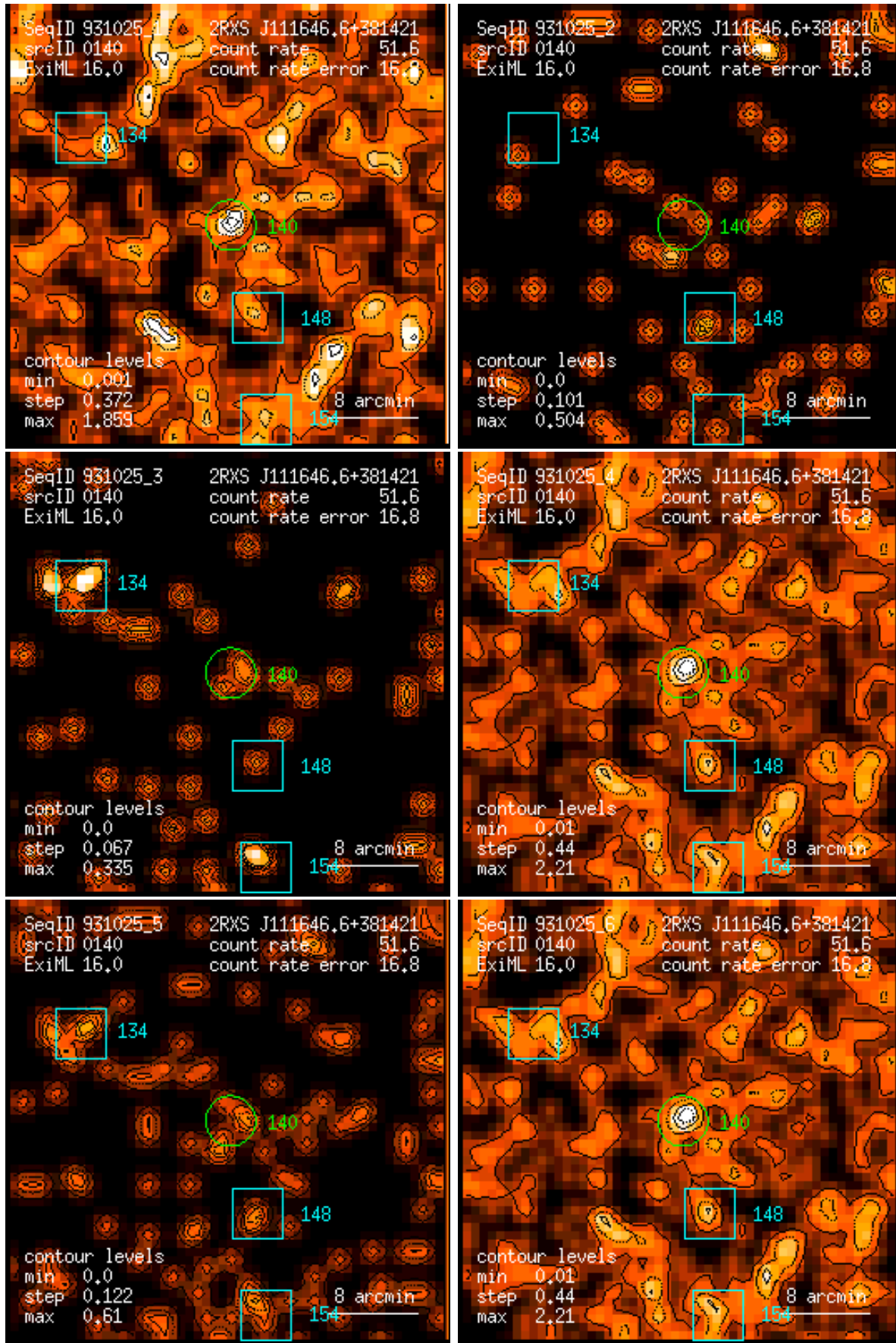
Figure 140: RASS 931025: detection 0140: band rate images, Gaussian filter: (1) PSPC channels 11 – 41, (2) 52 – 90, (3) 91 – 201, (4) 11 – 235, (5) 52 – 201, (6) 11 – 201. Broad band rates in counts/ks. Band rate contour levels in counts/ks/arcmin 2 .
